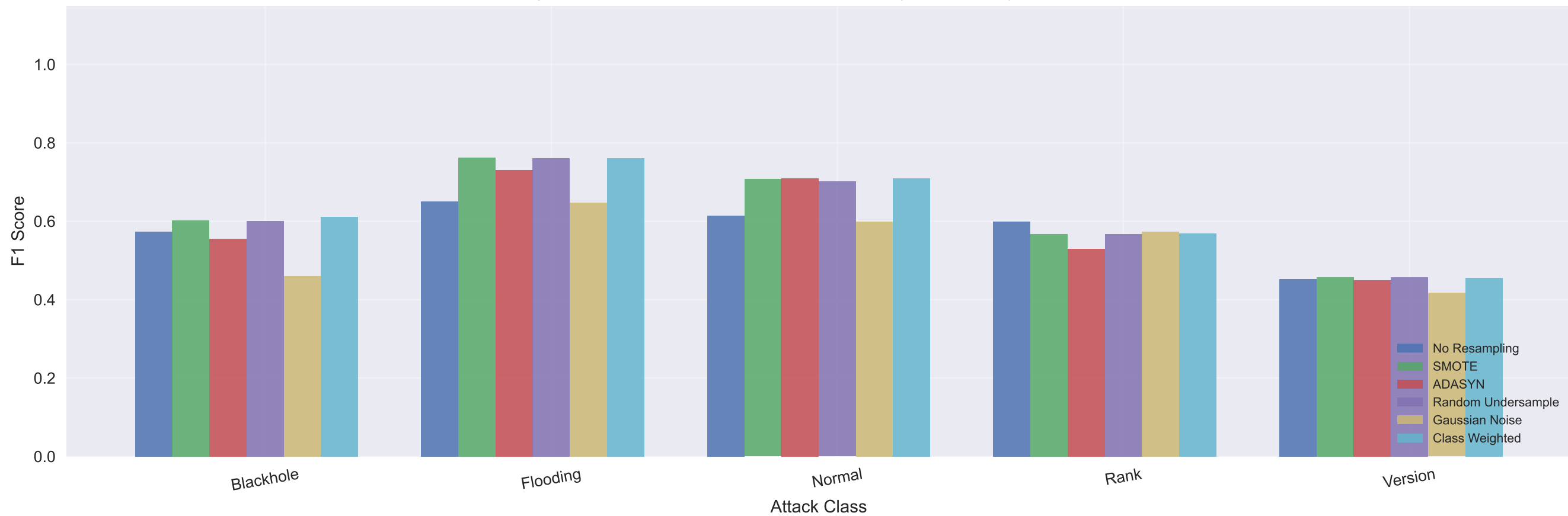
Figure 3: Per-Class F1 — Severe Imbalance (95% Normal) — XGBoost
