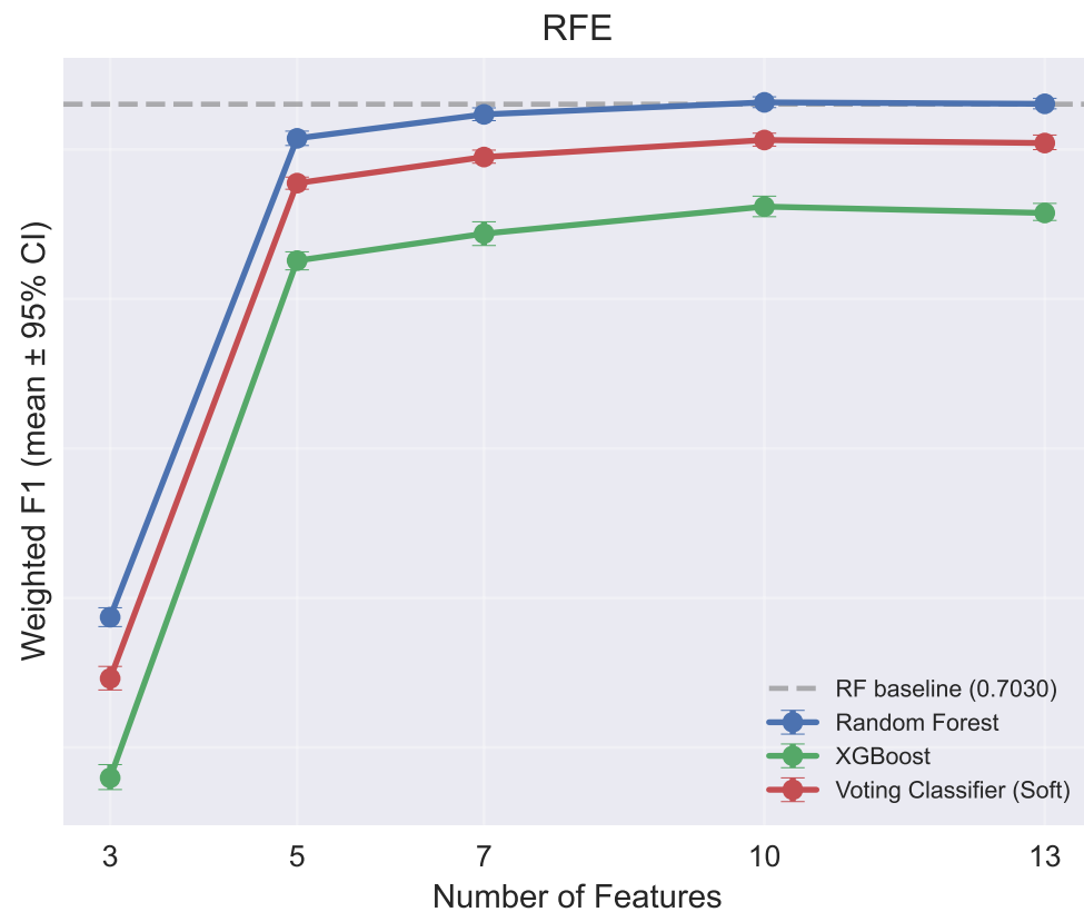
Figure 5: Weighted F1 vs Feature Subset Size Dashed = RF baseline (0.7030)
