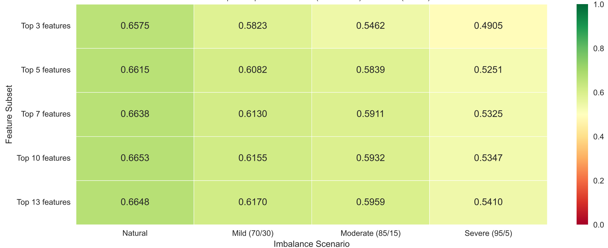
Figure 6: Mean Macro F1 — Feature Subset × Imbalance Scenario XGBoost | SHAP | Gaussian Noise (constructed) / Stratified (natural)
