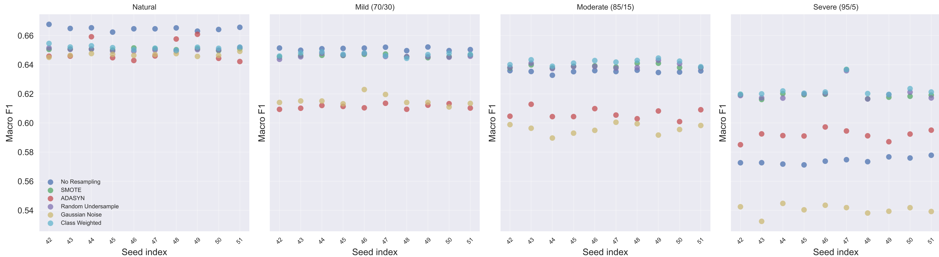
Figure 7: Per-Seed Macro F1 Scatter Variability across seeds
