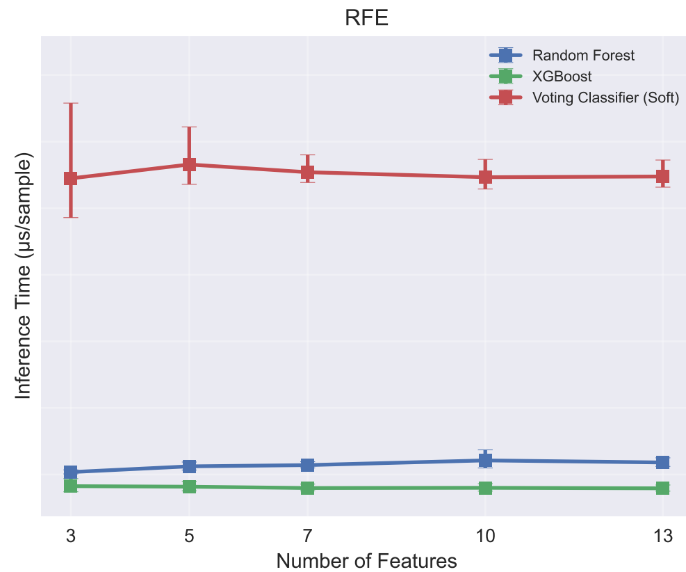
Figure 8: Inference Time vs Feature Subset Size Error bars = 95% bootstrap CI
