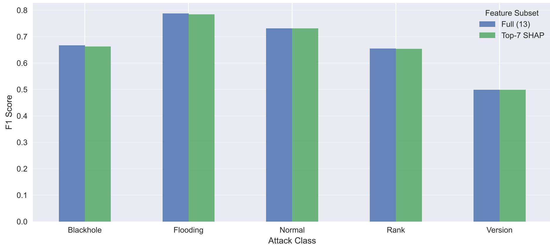
Per-Stratum F1: Full vs Top-7 SHAP Features XGBoost, Natural distribution
