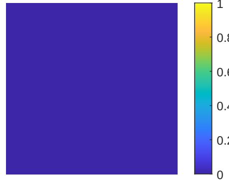
(h) \pi_b
