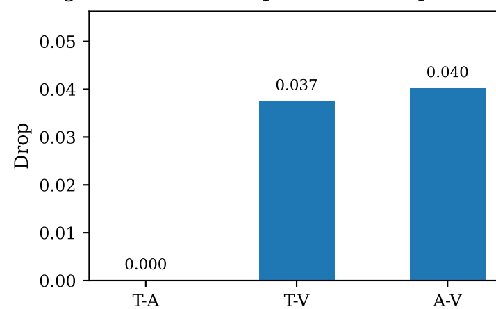
Alignment-score drop after visual perturbation
