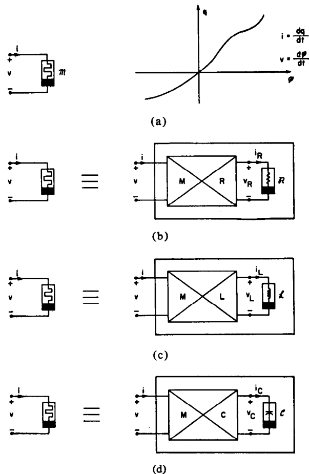
Fig. 1. Proposed symbol for memristor and its three basic realizations. (a) Memristor and its \phi - q curve. (b) Memristor basic realization 1: M - R mutator terminated by nonlinear resistor R . (c) Memristor basic realization 2: M - L mutator terminated by nonlinear inductor L . (d) Memristor basic realization 3: M - C mutator terminated by nonlinear capacitor C .
