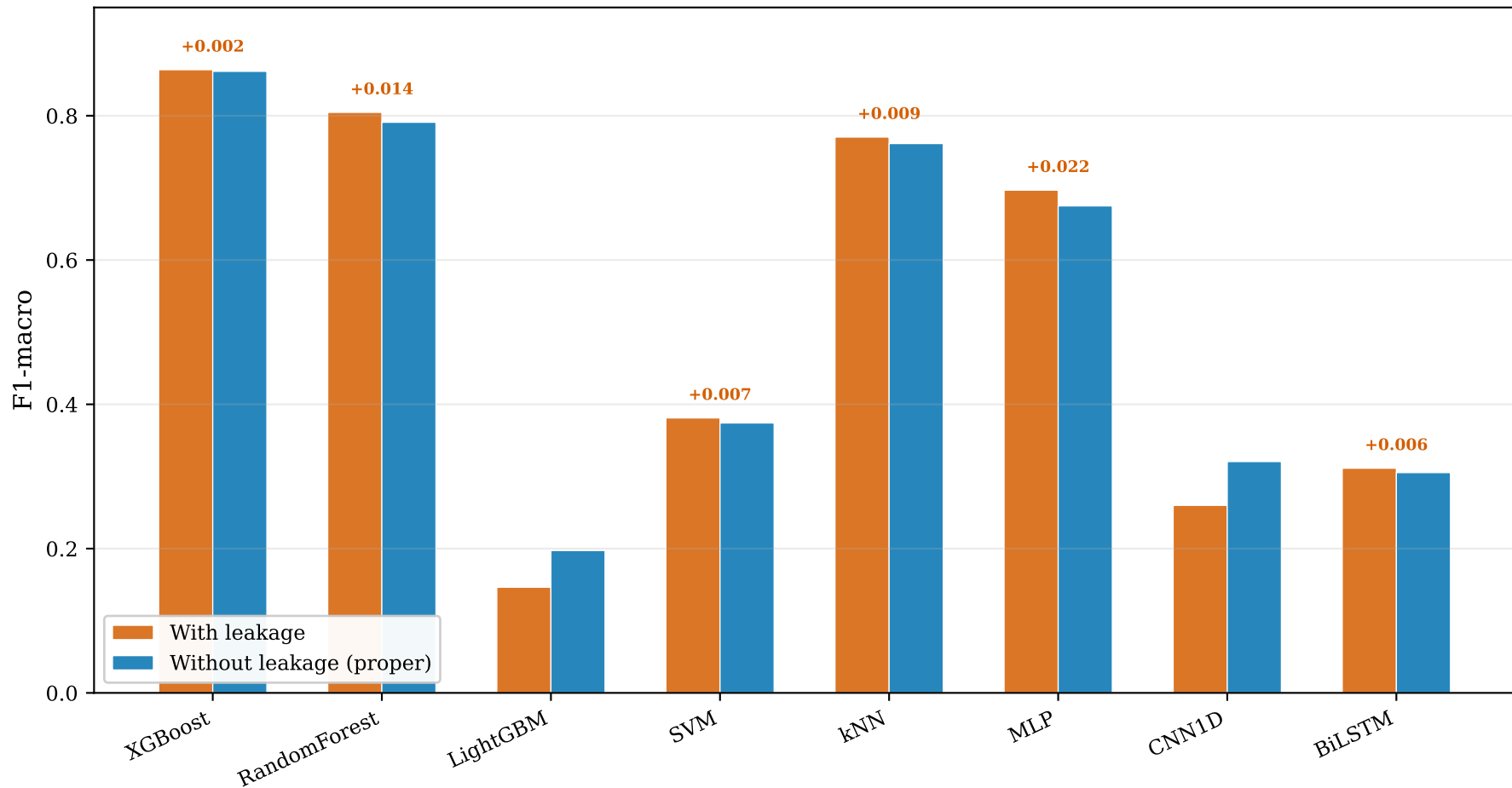
Data Leakage Impact — CICIDS2017 (Multi-class)
