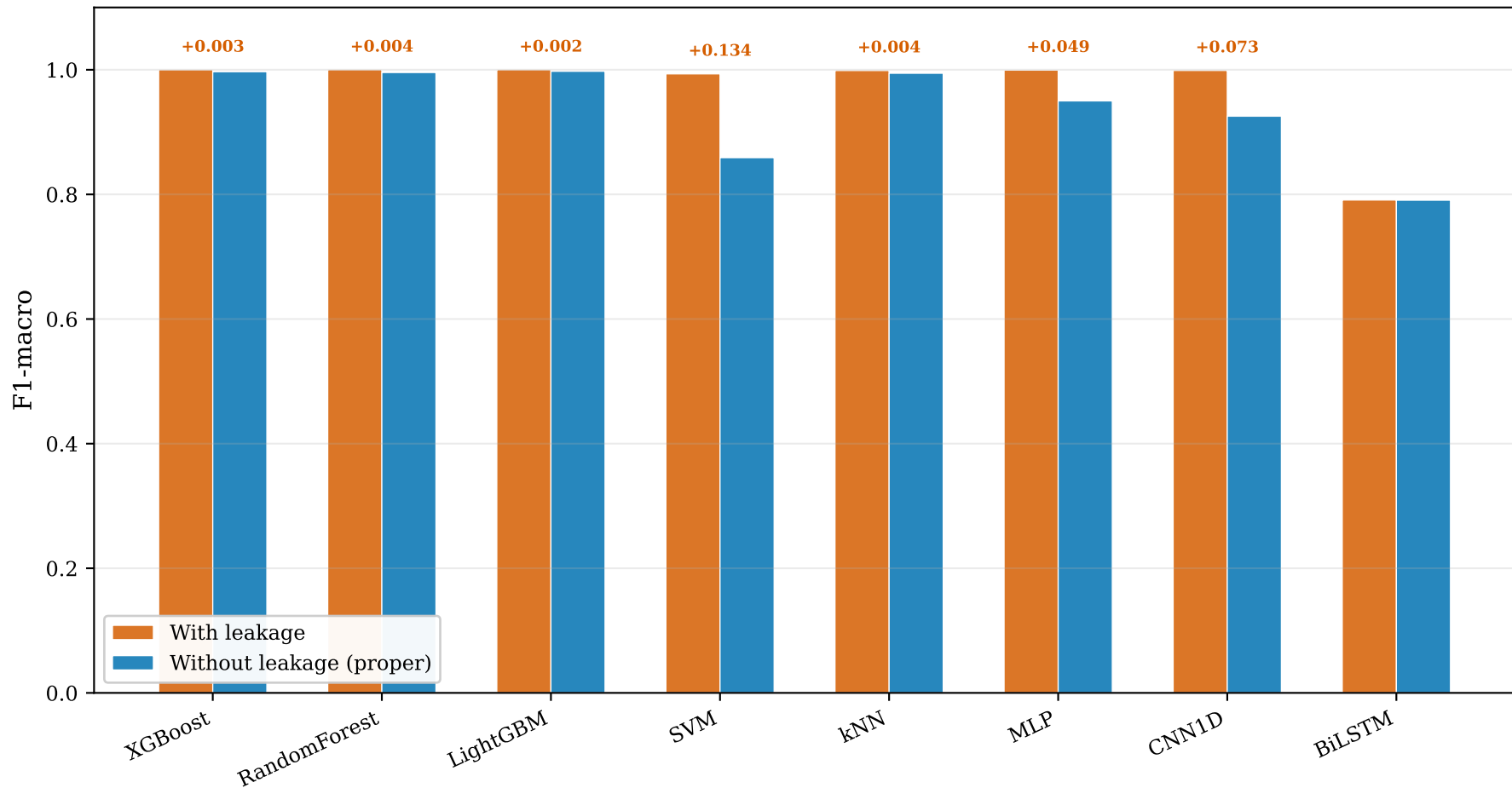
Data Leakage Impact — ToN-IoT (Binary)
