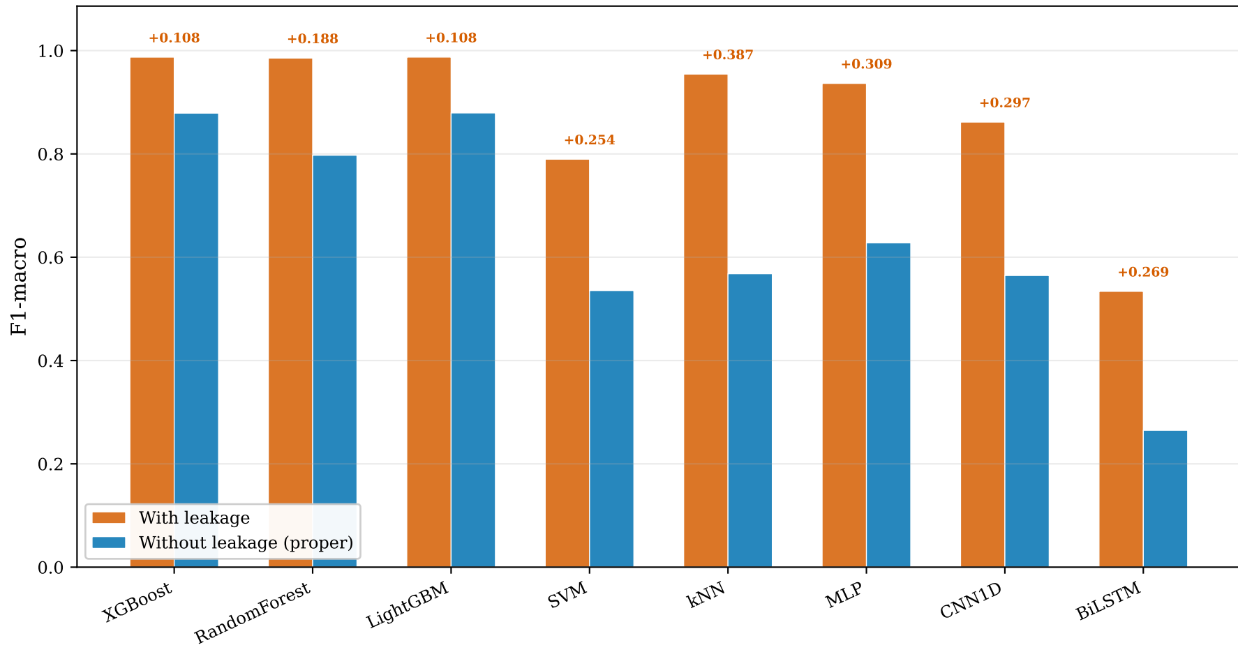
Data Leakage Impact — ToN-IoT (Multi-class)
