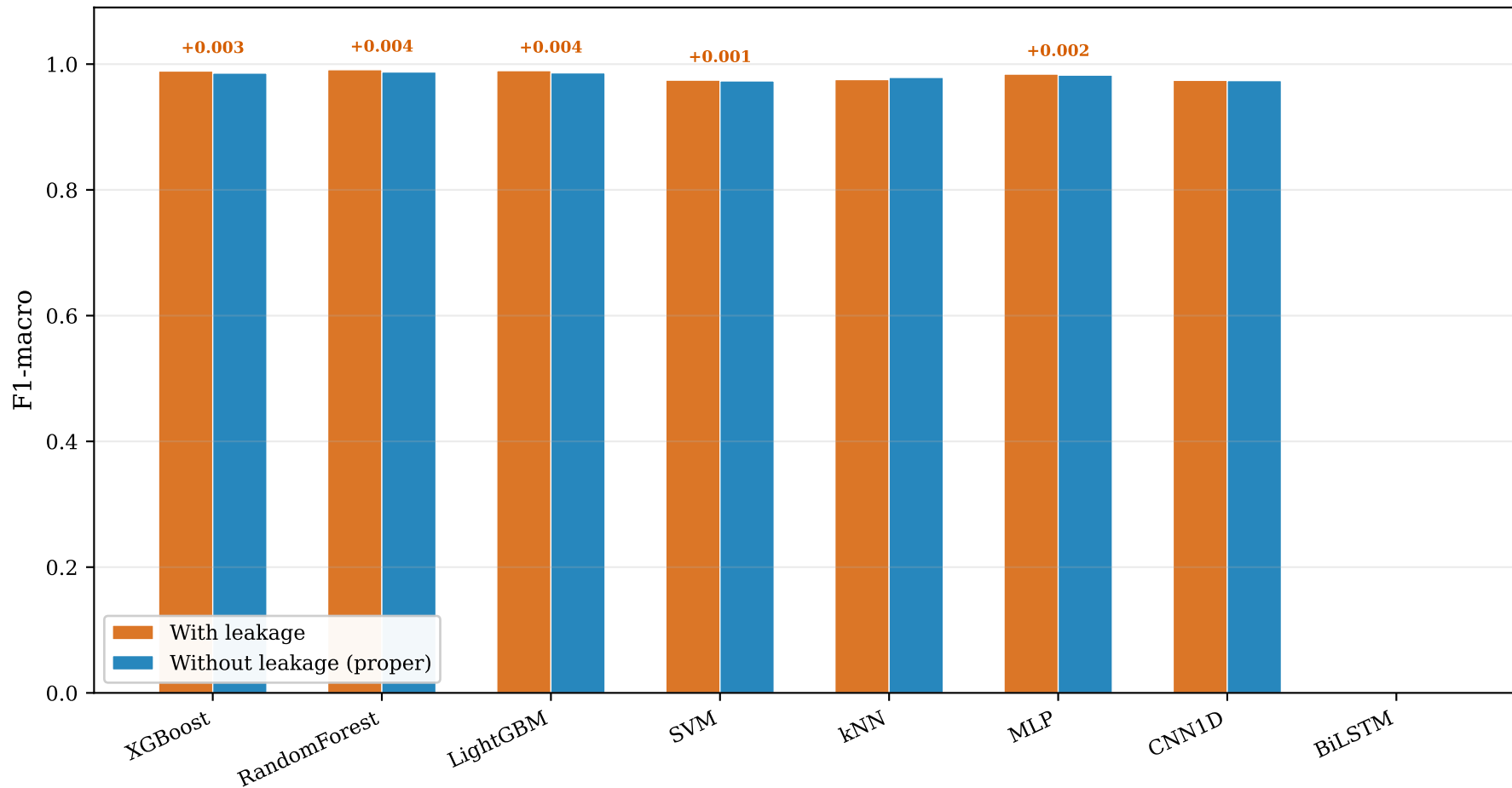
Data Leakage Impact — UNSW-NB15 (Binary)
