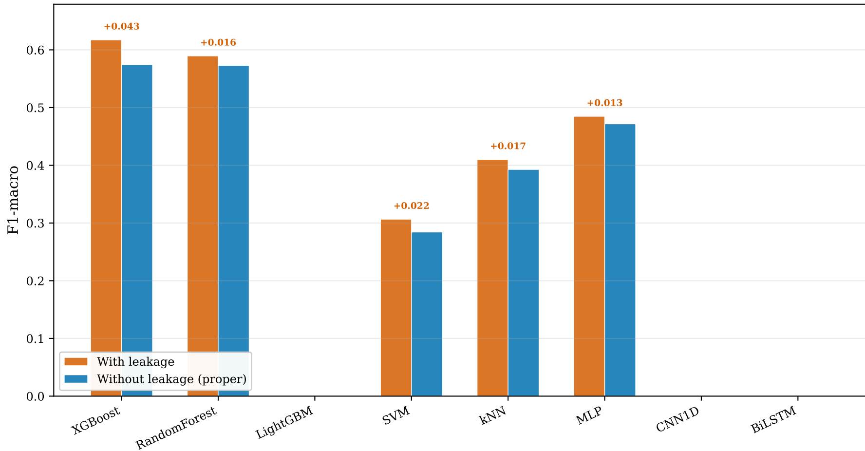
Data Leakage Impact — UNSW-NB15 (Multi-class)
