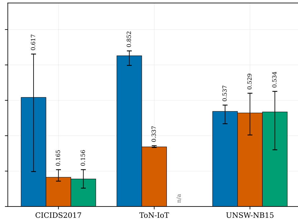
Multi-class classification
