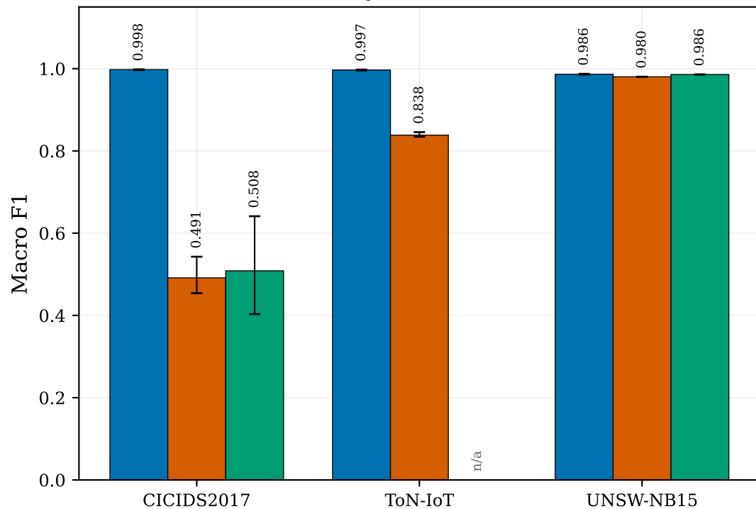
Binary classification
