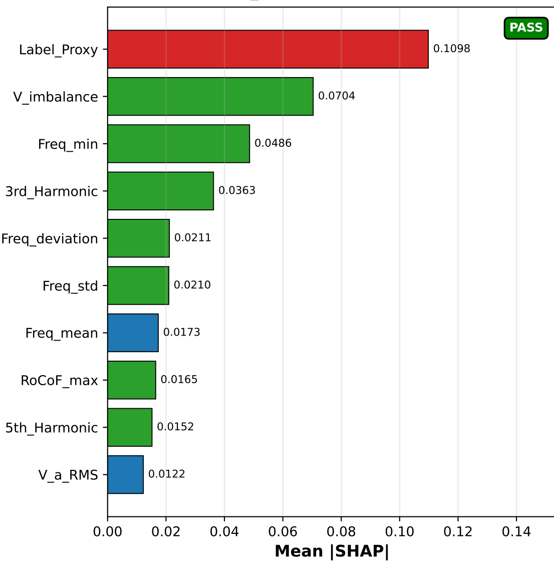
Corrupted Model A (+Label_Proxy, r \approx 0.89 with label)
