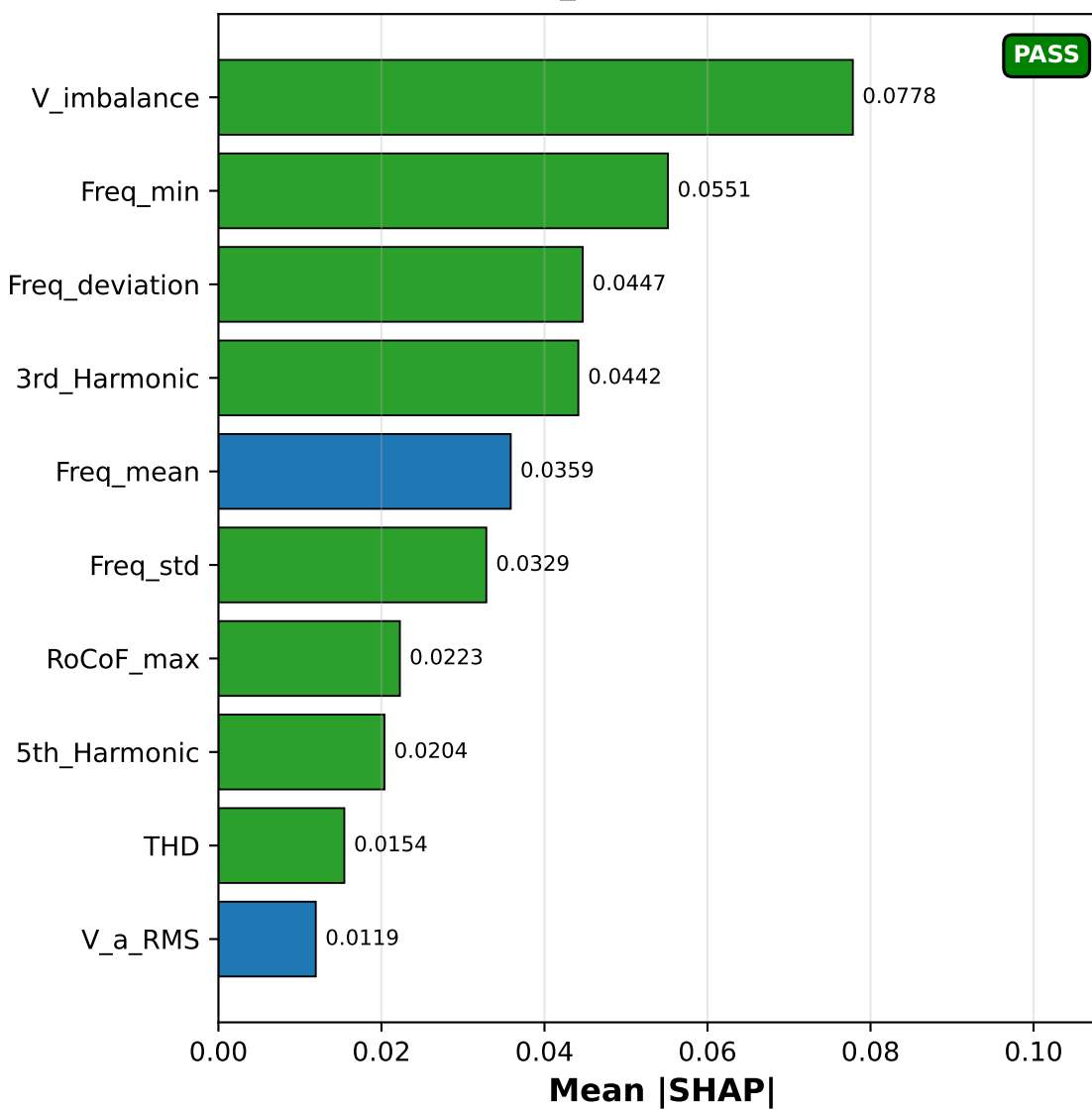
Corrupted Model B (+Random_Walk, r \approx 0 with label)
