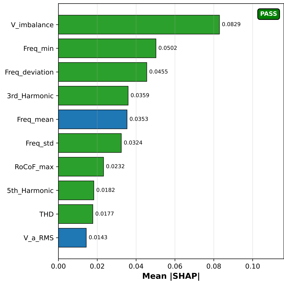
Clean Model (15 physics features only)
