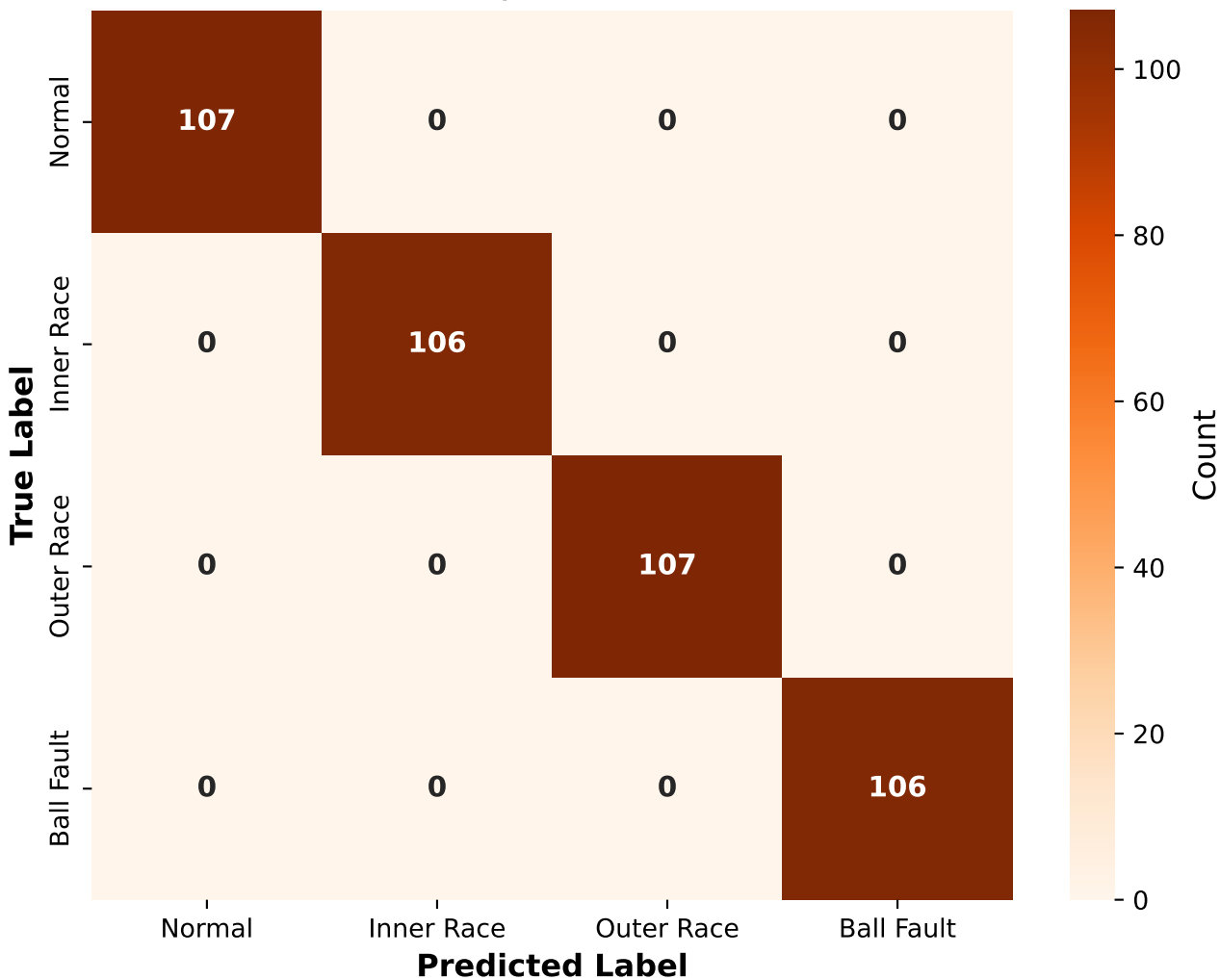
CWRU Real Data: Random Forest (acc=1.0000, n=426 windows)
