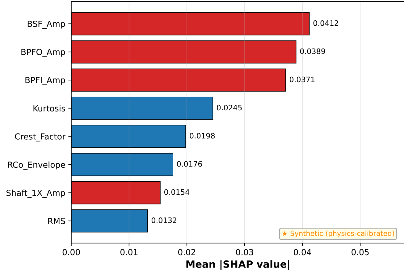
Synthetic Bearing Data (Parametric simulator, BPFI/BPFO features dominant)
