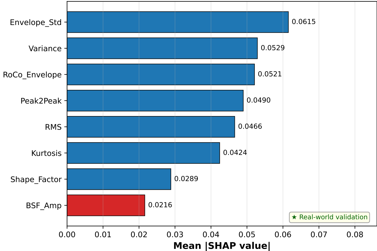
Real CWRU Bearing Data (Field vibration recordings, same pipeline, no tuning)
