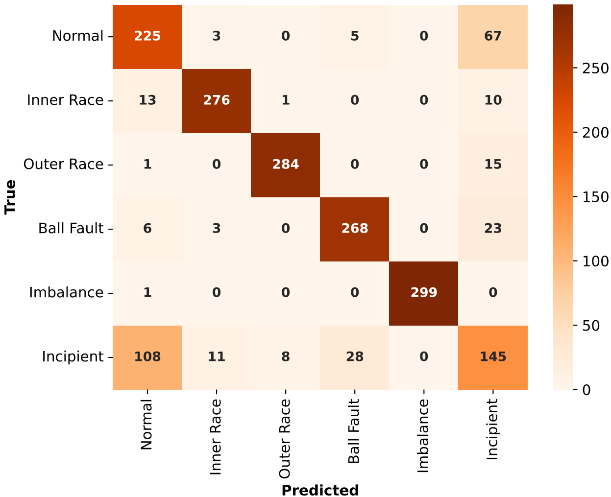
Bearing Confusion Matrix: Decision Tree (test n=1,800, acc=0.8317)
