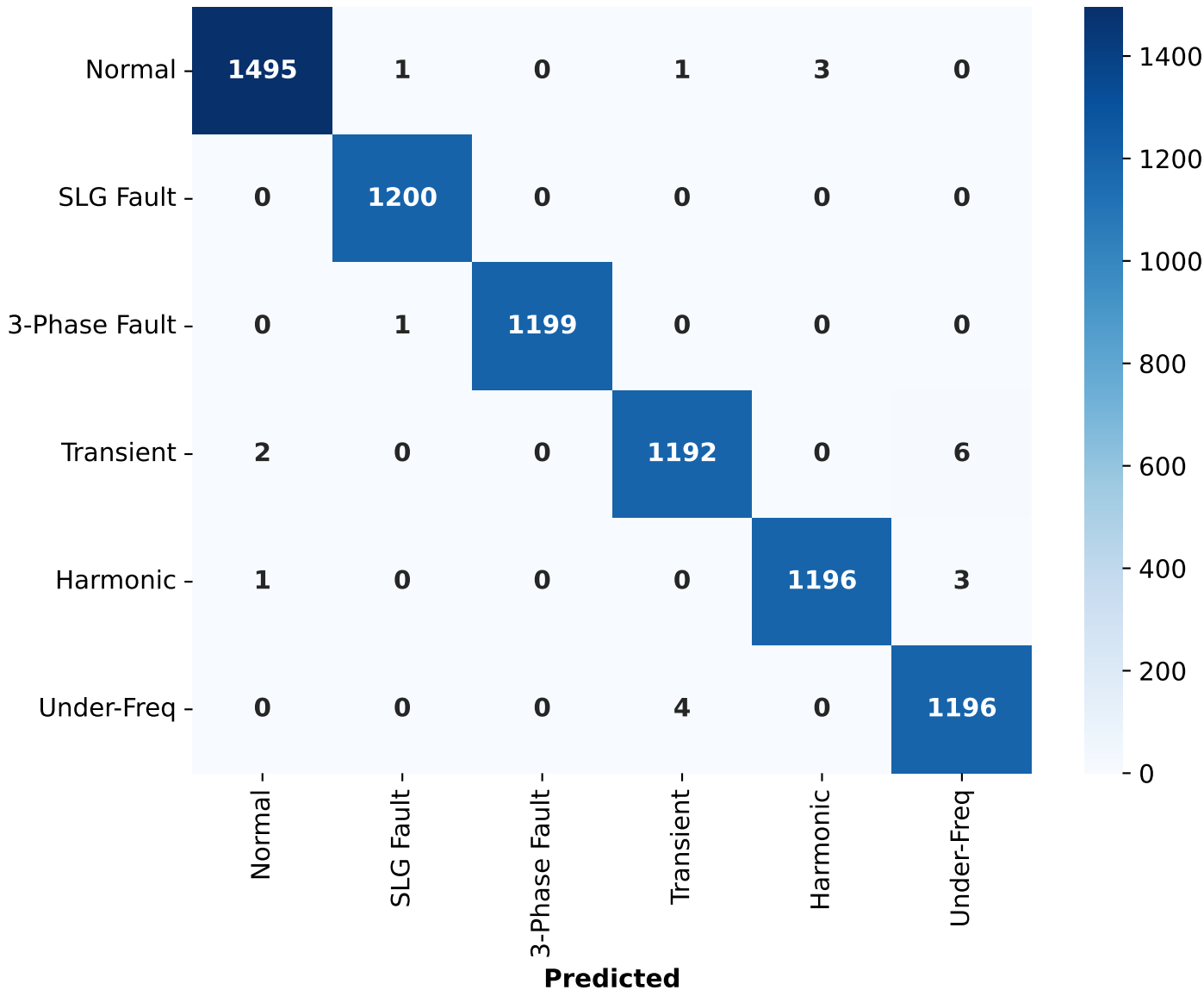
1D-CNN Confusion Matrix (test n=7,500, acc=0.9971)
