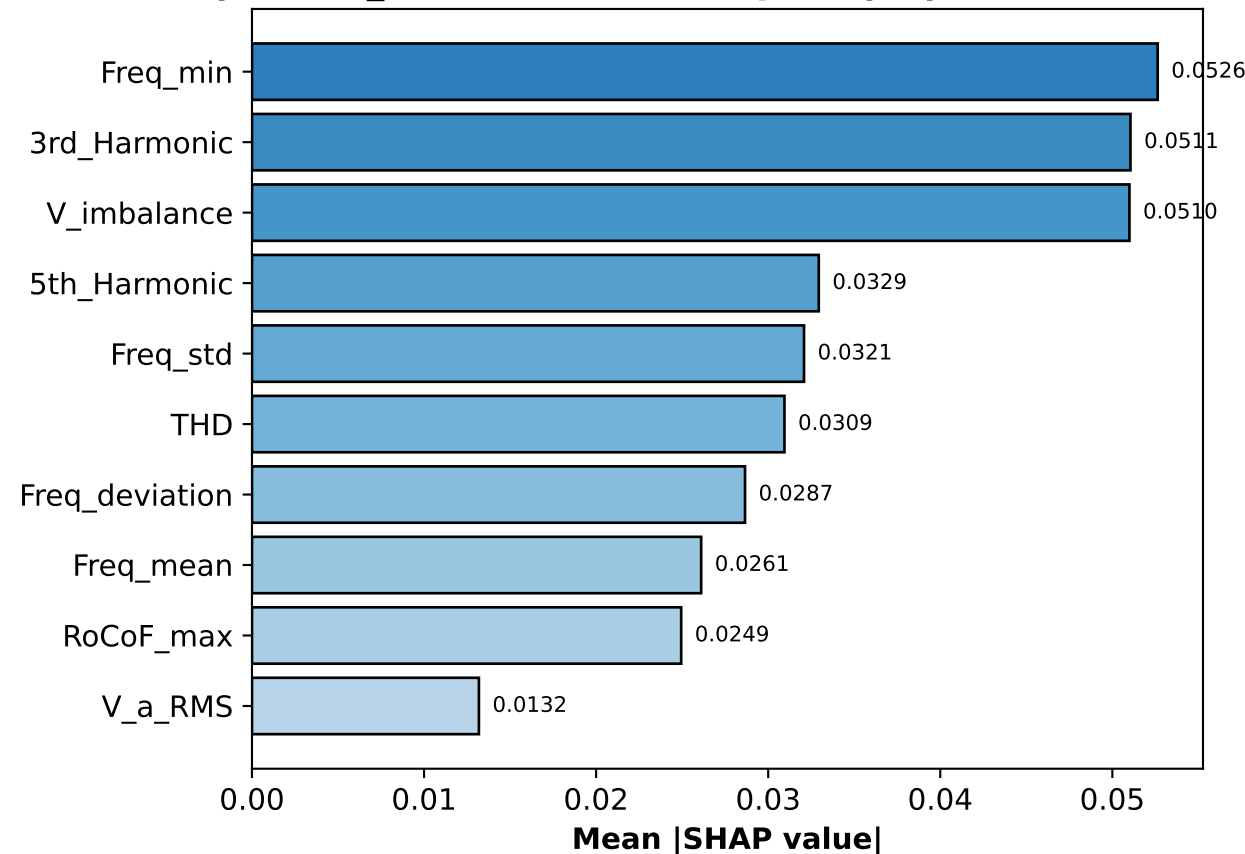
Domain A: Power Grid (Physics: V_imbalance and frequency dynamics dominate)
