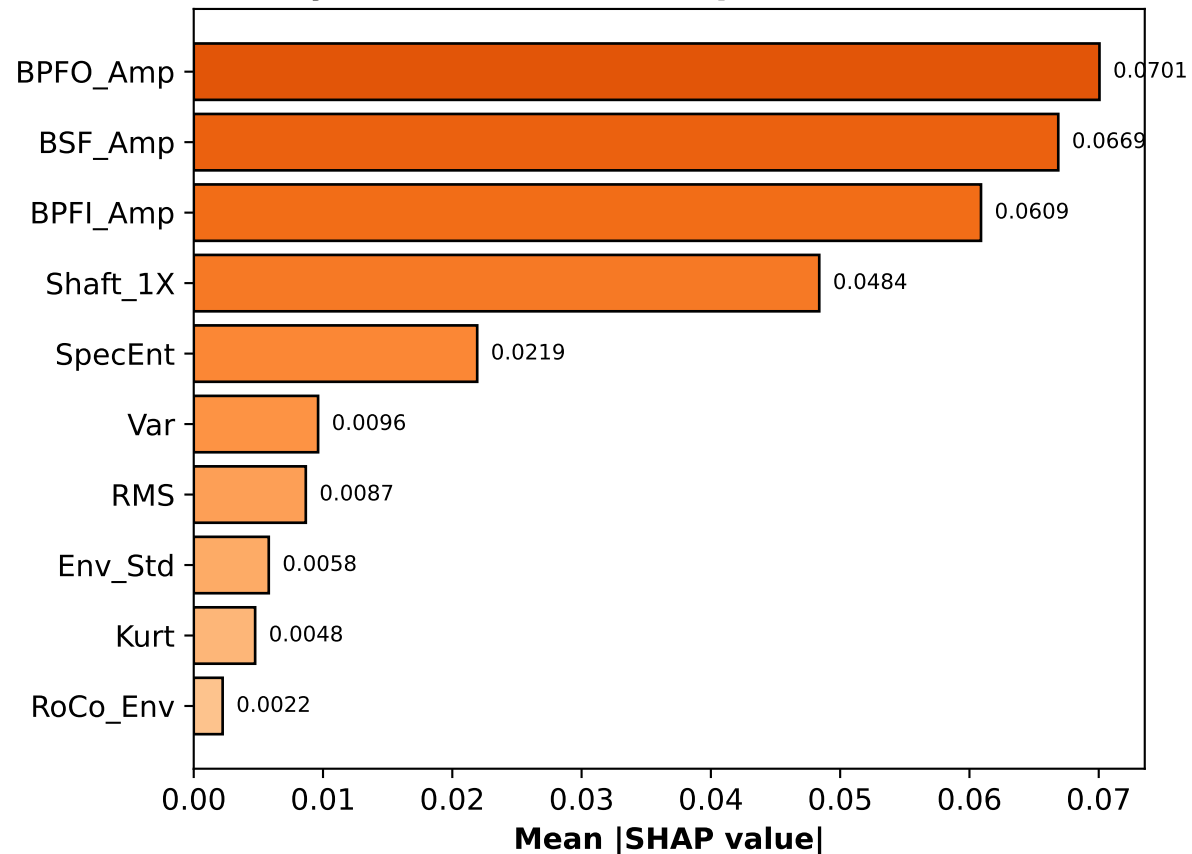
Domain B: Industrial Bearing (Physics: BPFI/BPFO amplitudes dominate)
