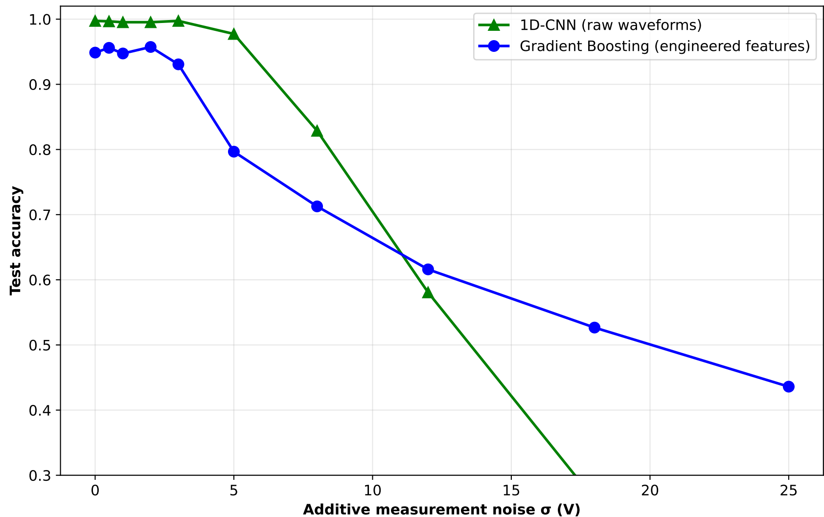
Noise robustness: raw-waveform CNN vs feature-based baseline
