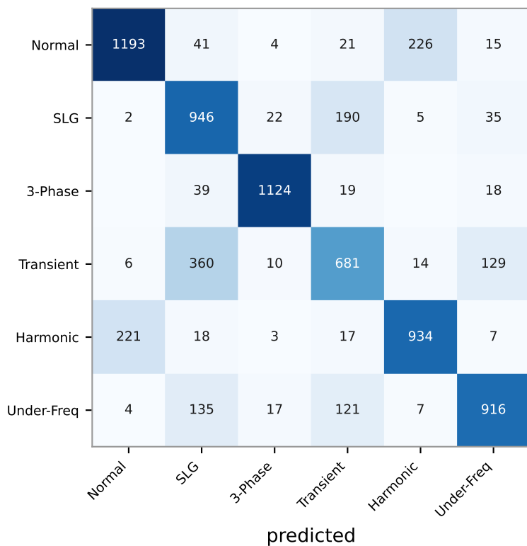
XGBoost (77.3%)
