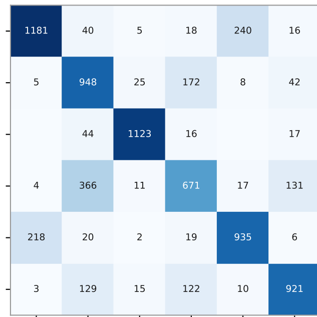
Random Forest (74.2%)
