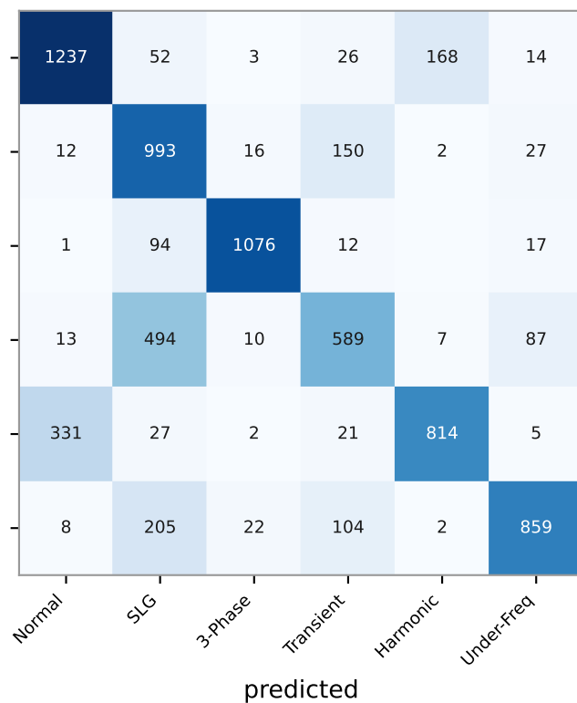
Random Forest (74.2%)
