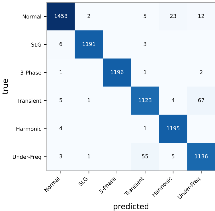
1D-CNN (seed 42, acc 97.3%)
