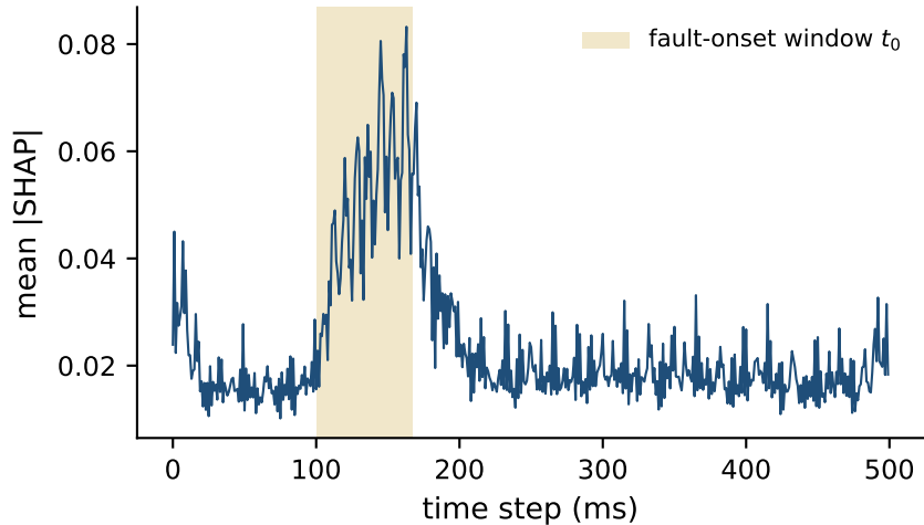
Per-time-step attribution
