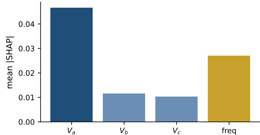
Per-channel attribution
