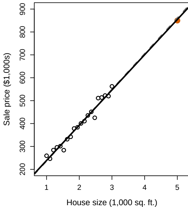
High leverage, not influential
