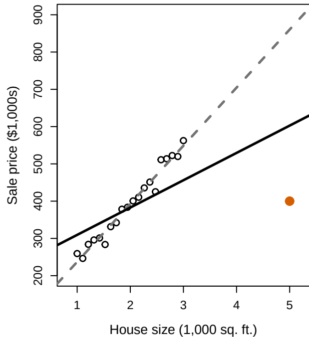
High leverage and influential
