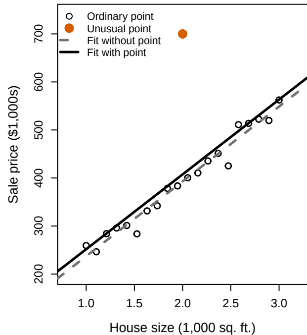
Response outlier, low leverage
