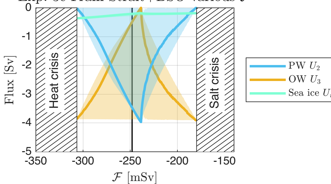
Exp. 3c Fram Strait+BSO various \mathcal{F}
