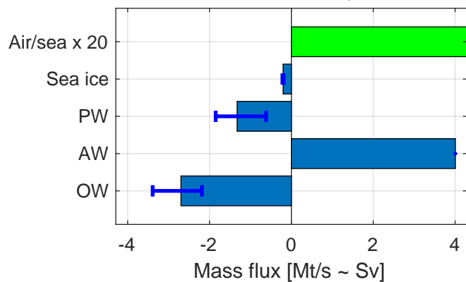
Polar Fluxes, A
