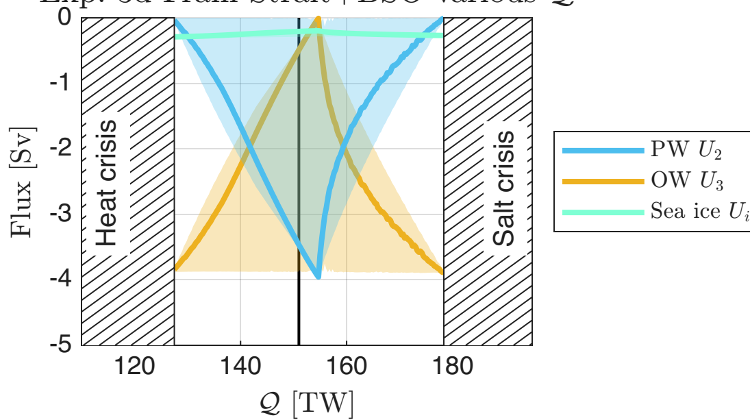
Exp. 3d Fram Strait+BSO various Q
