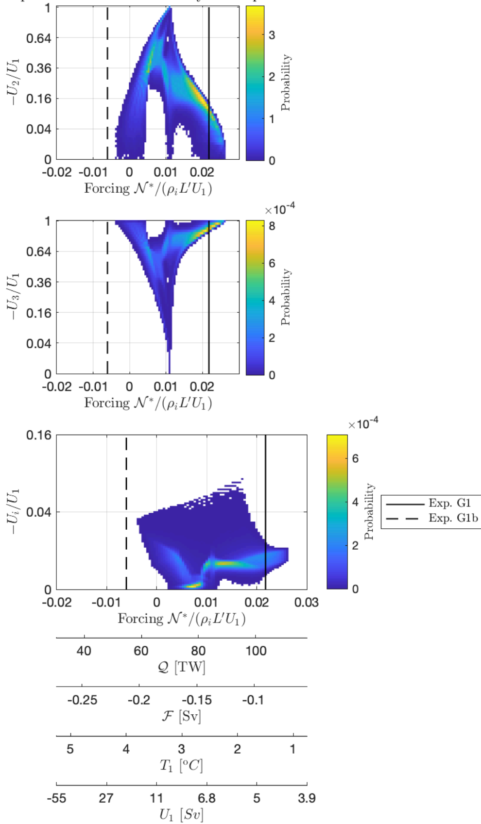
Exp. G4 Arctic LGM sensitivity wrt Expt. G1
