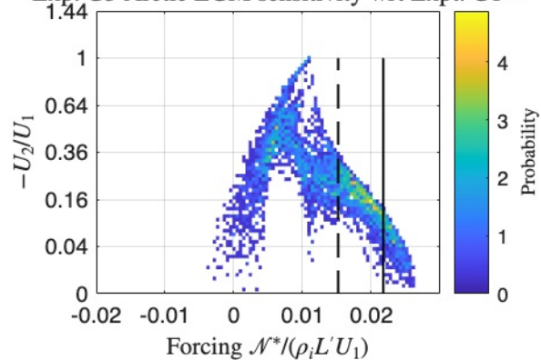
Exp. G3 Arctic LGM sensitivity wrt Expt. G1 \times 10^{-4}
