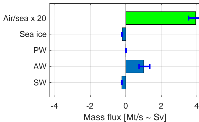
Shelf Fluxes, B
