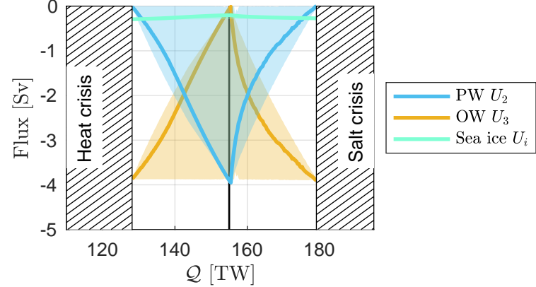
Exp. 3d Fram Strait+BSO various Q
