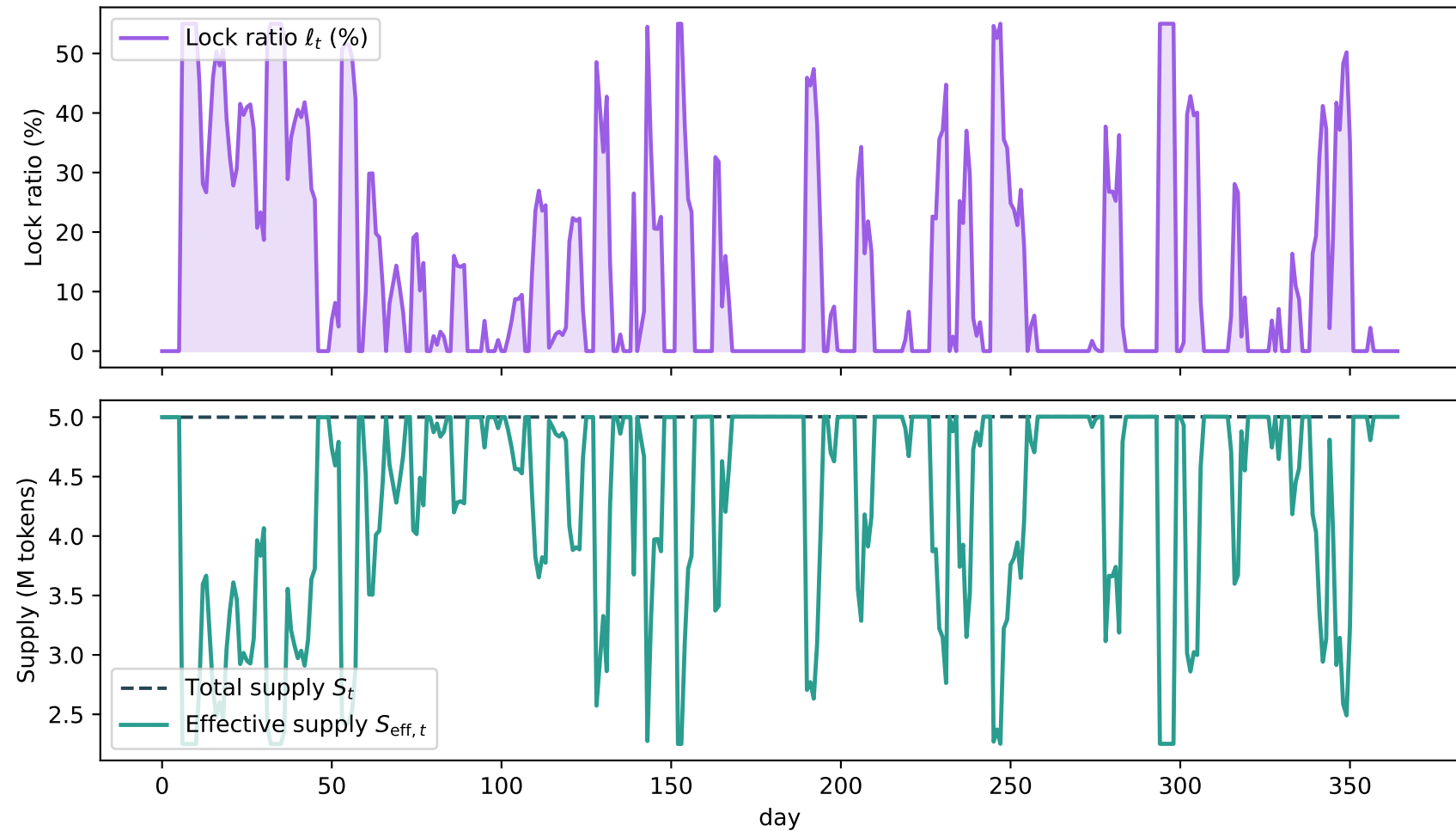
Figure 6. Volatility-triggered lock ratio and effective supply
