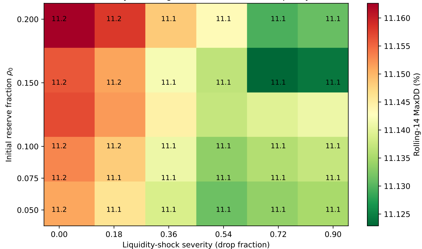
Failure boundary — rolling-14 MaxDD (%) under liquidity shock
