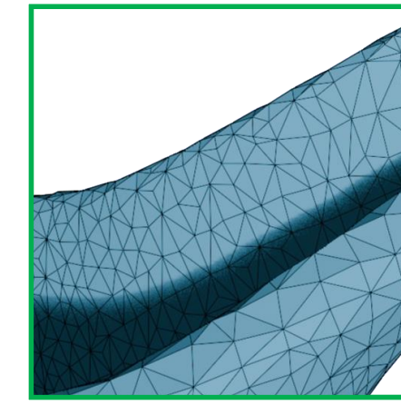
FlexiCubes (128×128×128) 120K Tris 4.33Mb
