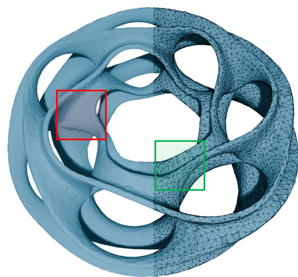
SH-Cubes (64×64×64) 15K Tris 1.08Mb
