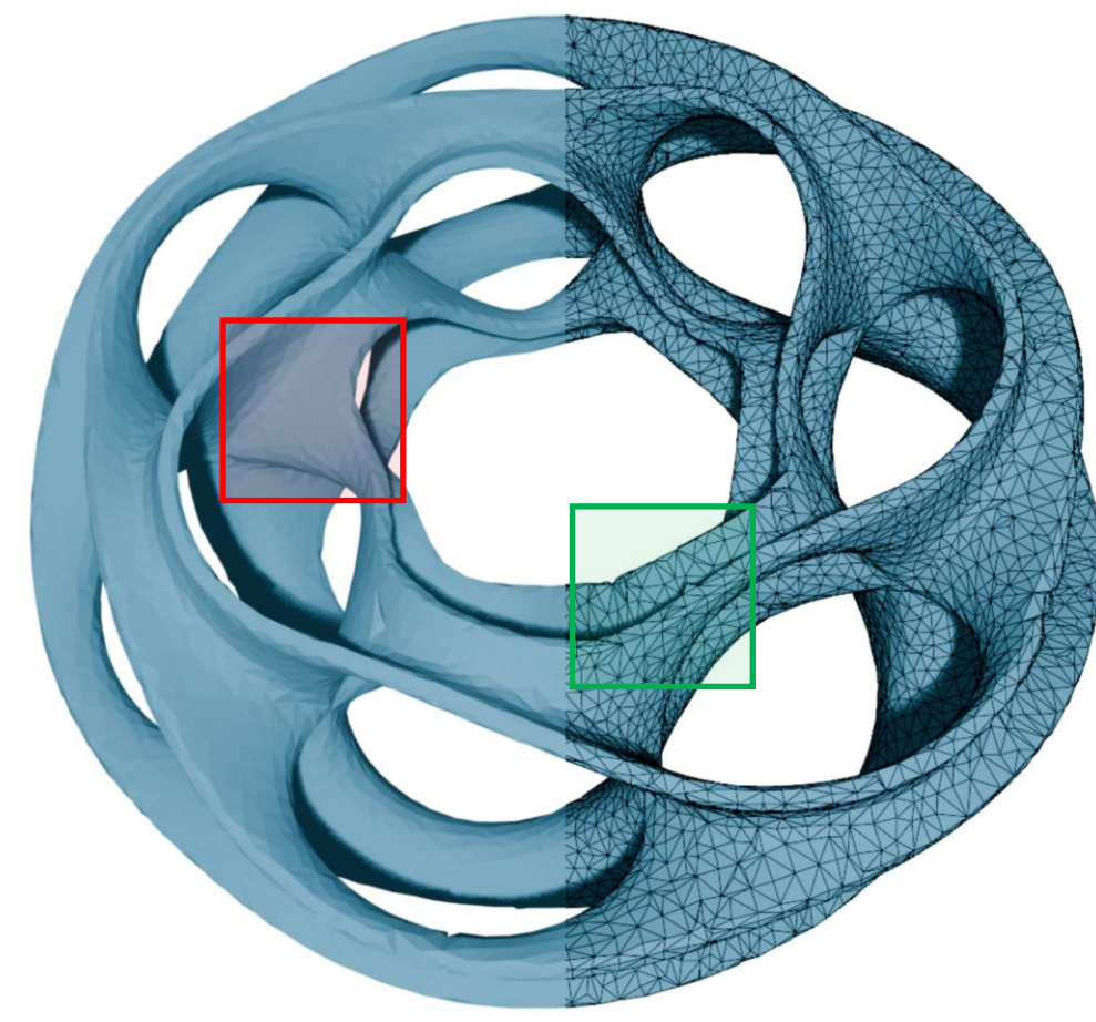
FlexiCubes (64×64×64) 15K Tris 1.08Mb
