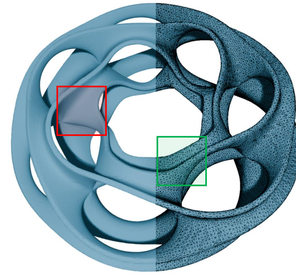
FlexiCubes (128×128×128) 120K Tris 4.33Mb
