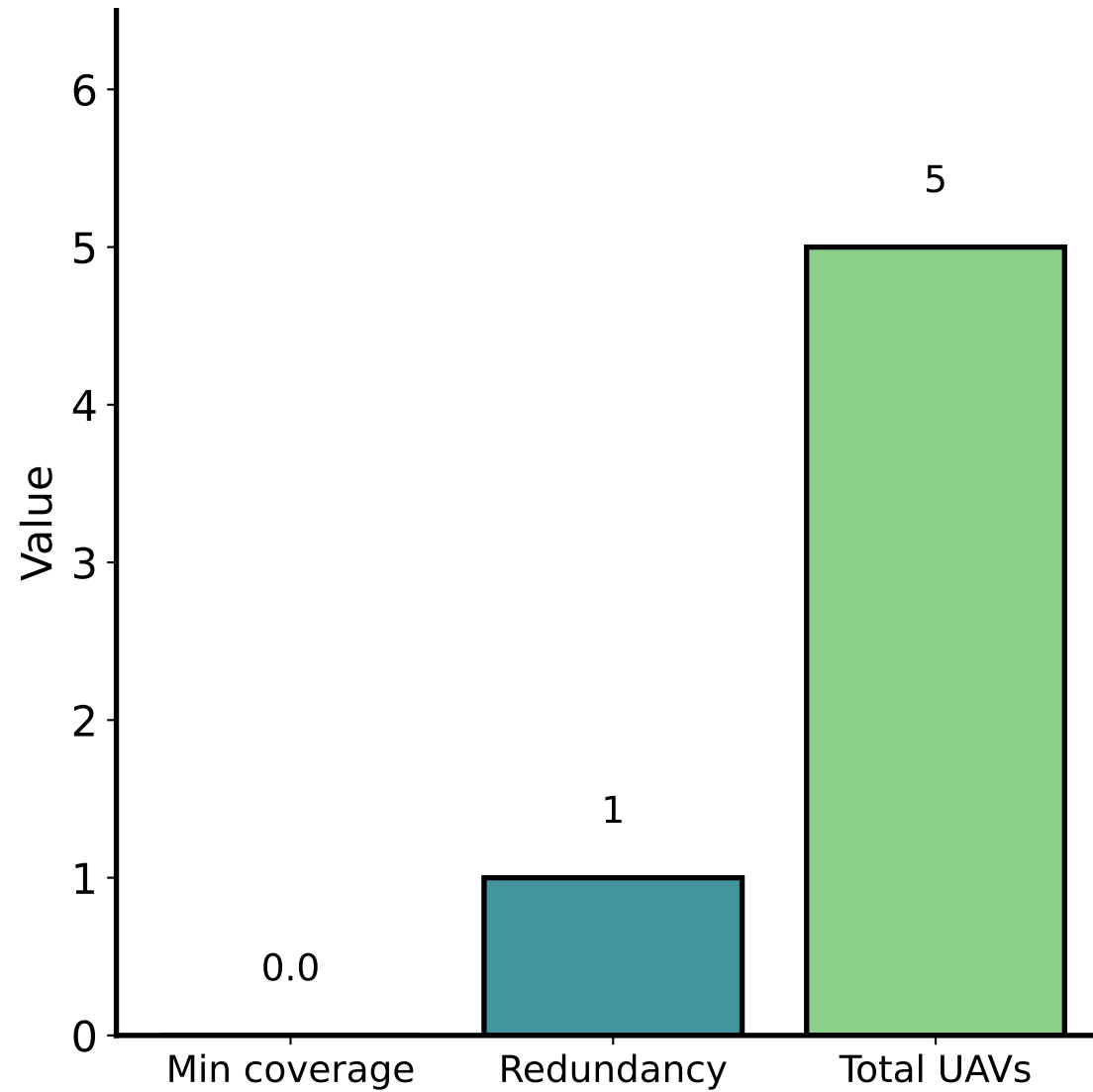
Robust metrics
