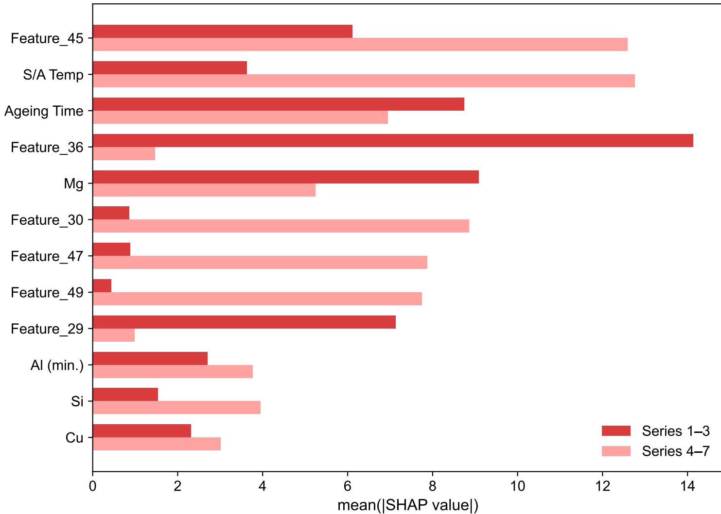
YTS — SHAP Grouped Importance
