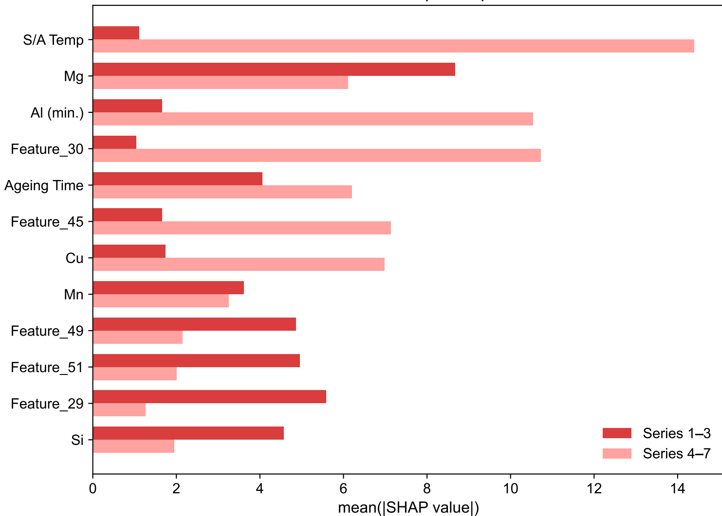
UTS — SHAP Grouped Importance
