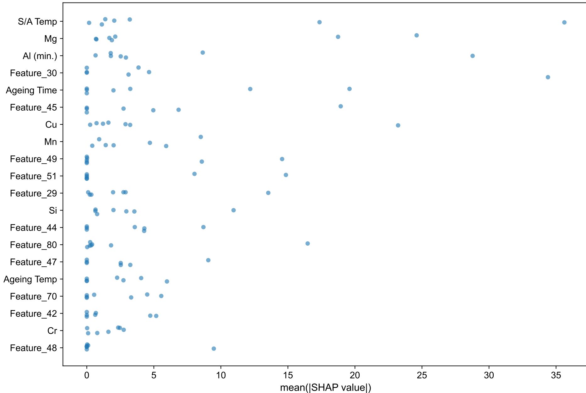
UTS — Series-level Beeswarm SHAP
