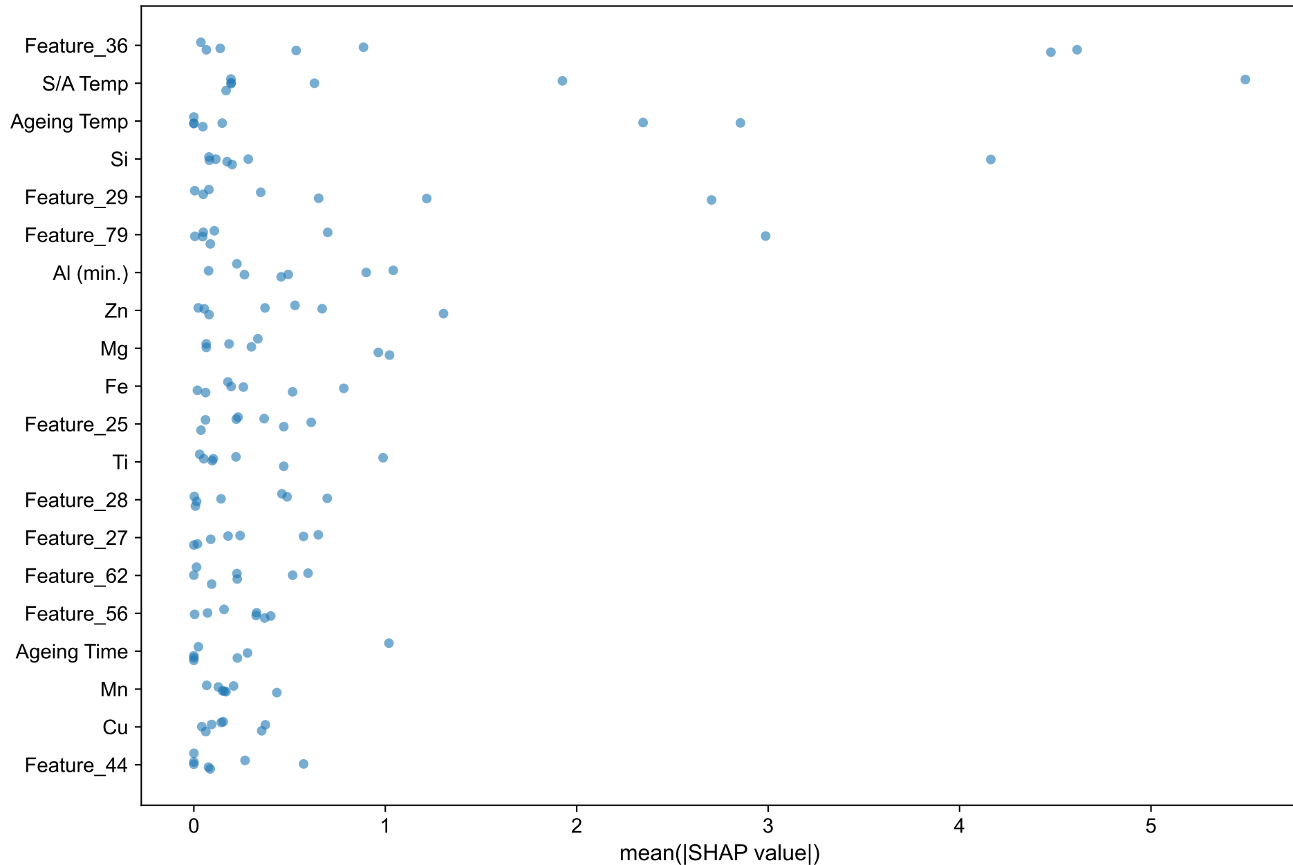
EL — Series-level Beeswarm SHAP
