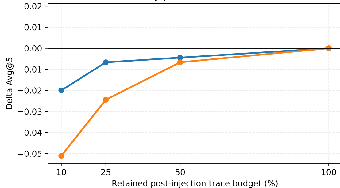
Latency-prioritized vs random
