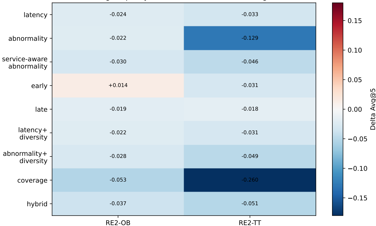
Stage A policy delta vs random at 10% budget
