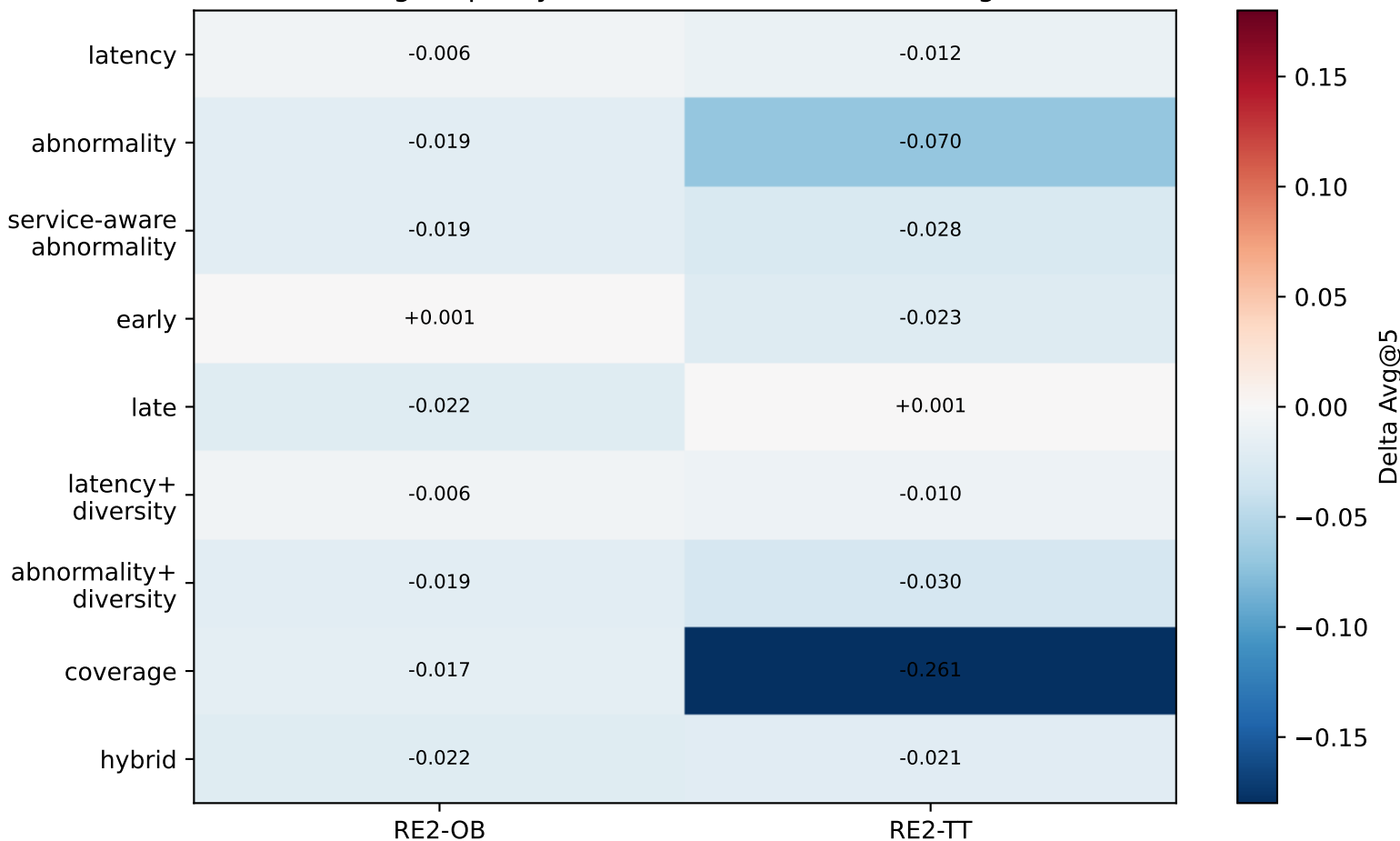
Stage A policy delta vs random at 25% budget
