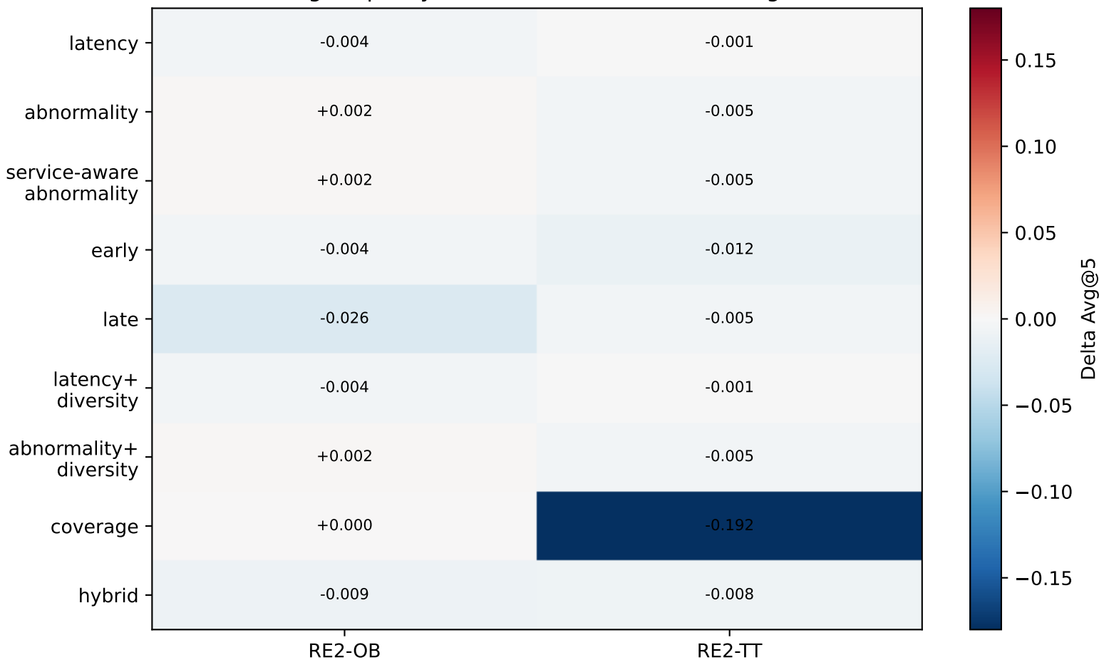
Stage A policy delta vs random at 50% budget
