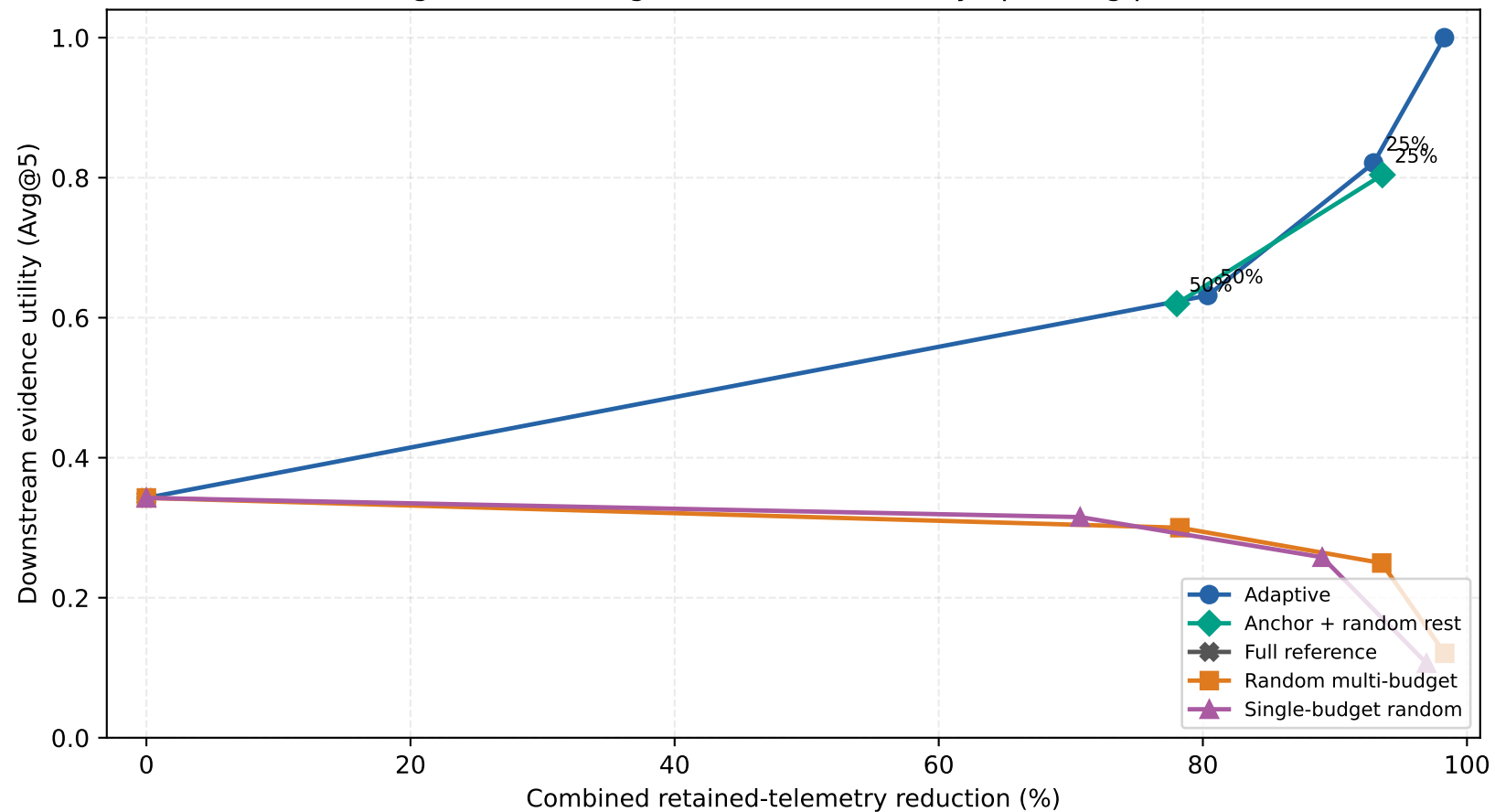
Stage B monitoring-cost / evidence-utility operating points
