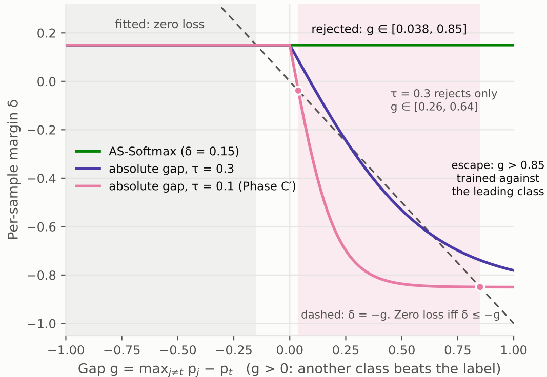
(a) Absolute gap, s = \sigma(g / \tau) , \beta = 1
