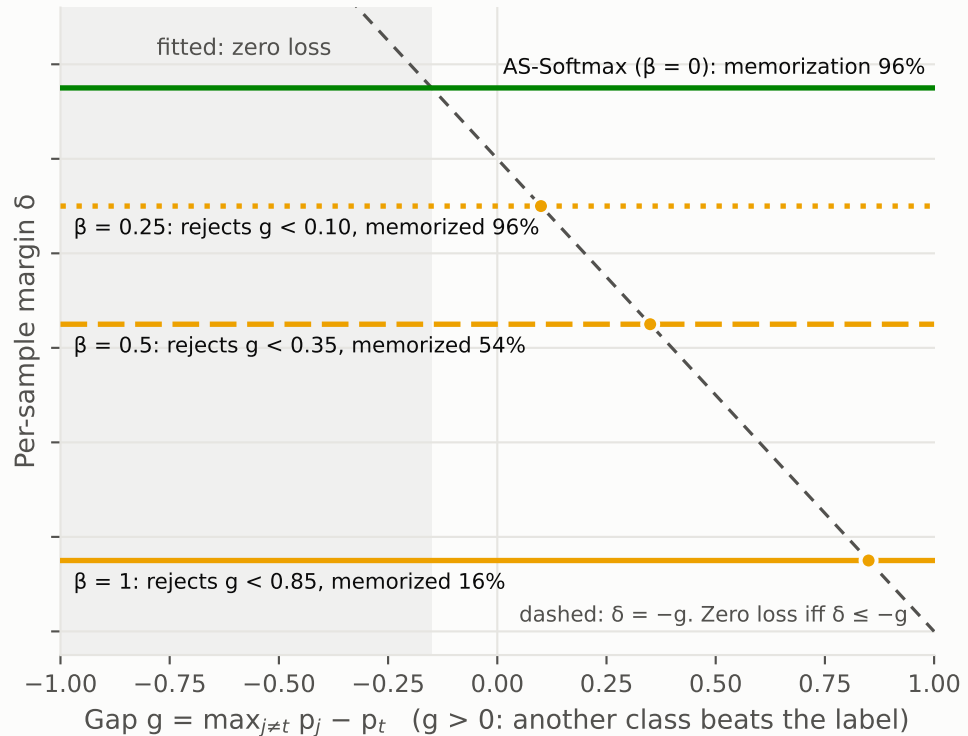
(b) Batch-relative M4: the floor \delta_b - \beta caps the rejectable gap
