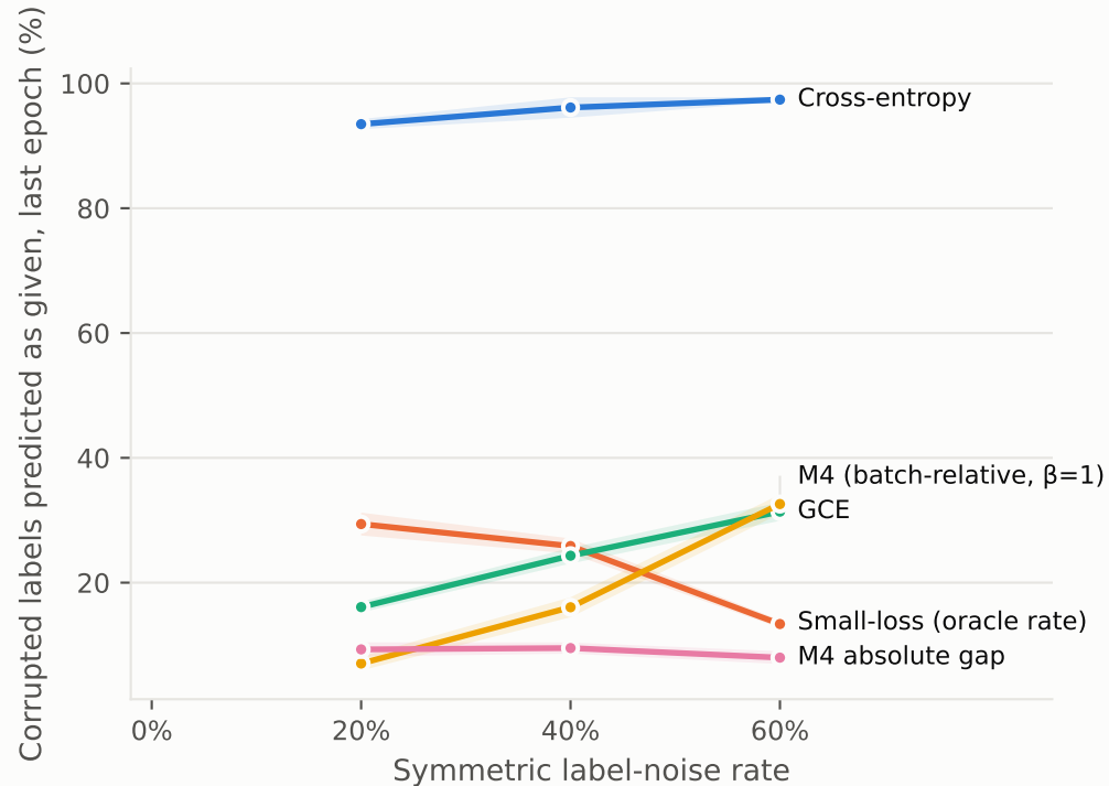
20 Newsgroups, BERT-base, 8 epochs, 5 seeds (mean \pm sd). Right: no corrupted labels at 0%.
