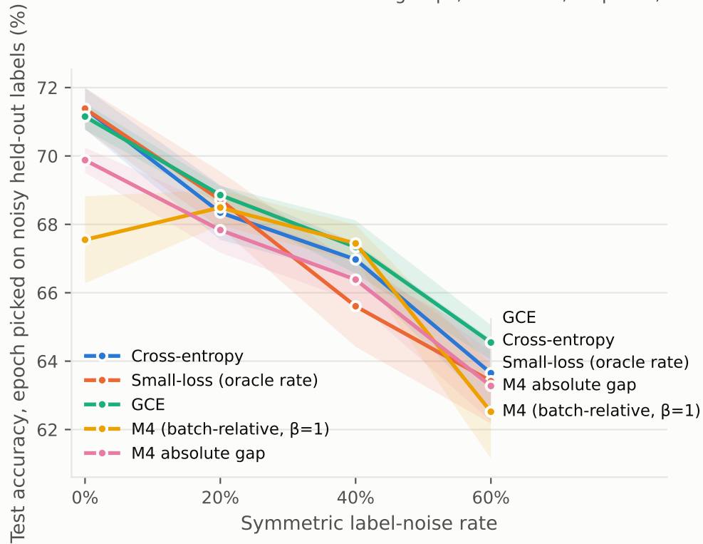
20 Newsgroups, BERT-base, 8 epochs, 5 seeds (mean \pm sd). Right: no corrupted labels at 0%.
