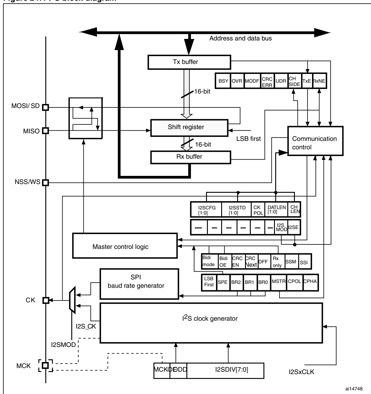
Figure 247. I 2 S block diagram
