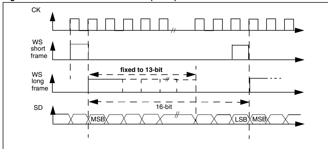
Figure 263. PCM standard waveforms (16-bit)
