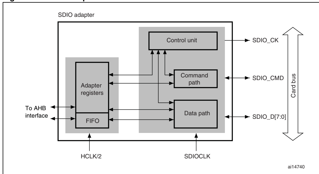
Figure 212. SDIO adapter
