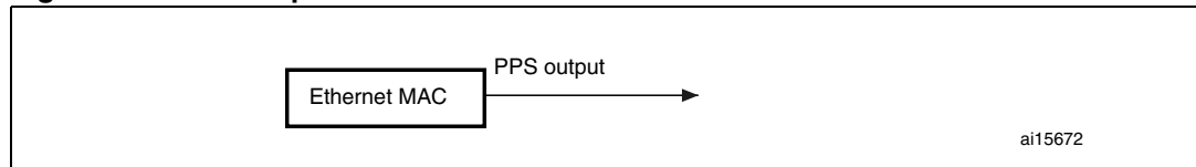
Figure 350. PPS output
