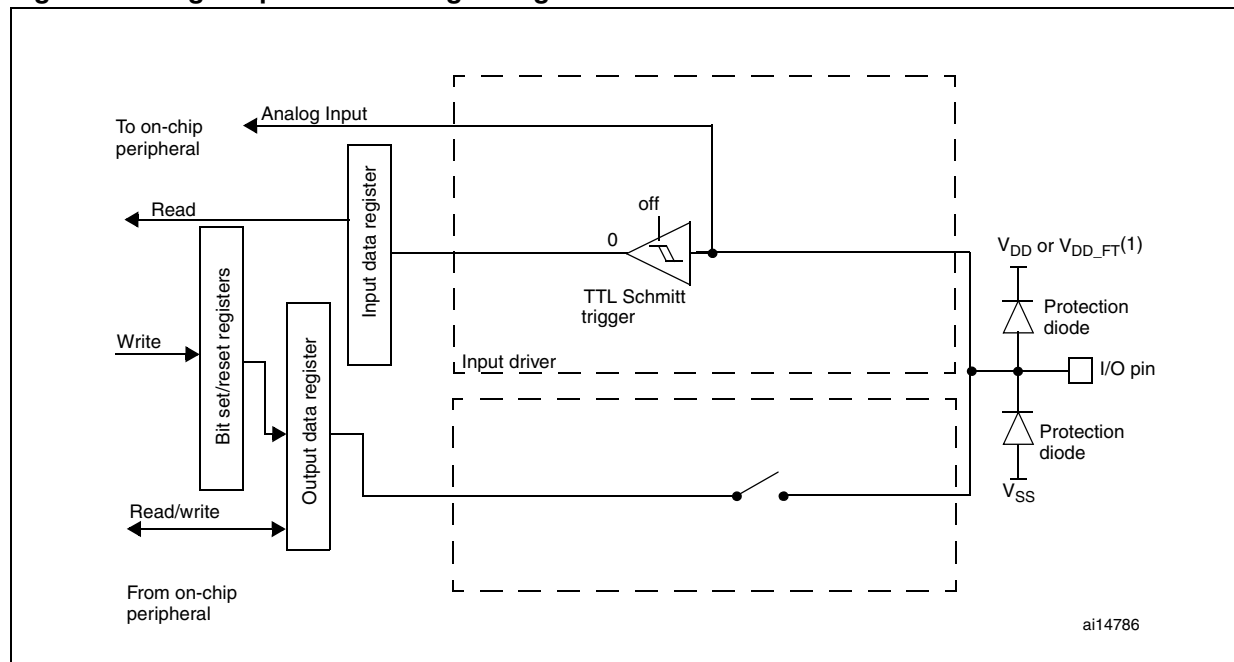
Figure 18. High impedance-analog configuration
