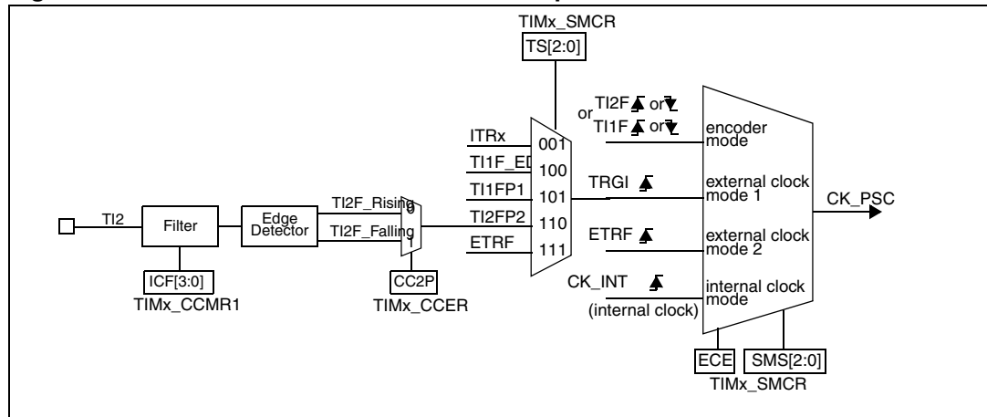
Figure 121. TI2 external clock connection example
