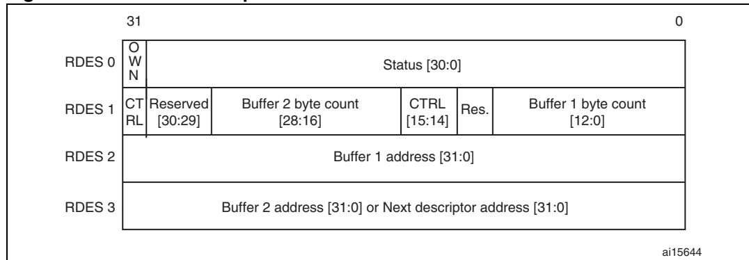
Figure 356. Rx DMA descriptor structure
