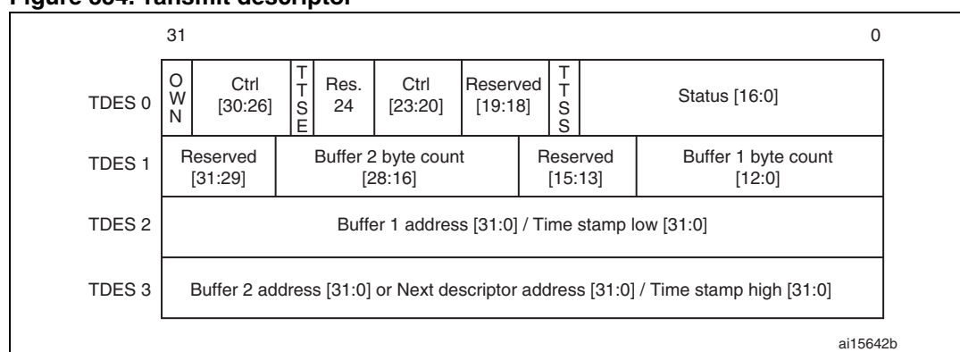
Figure 354. ransmit descriptor
