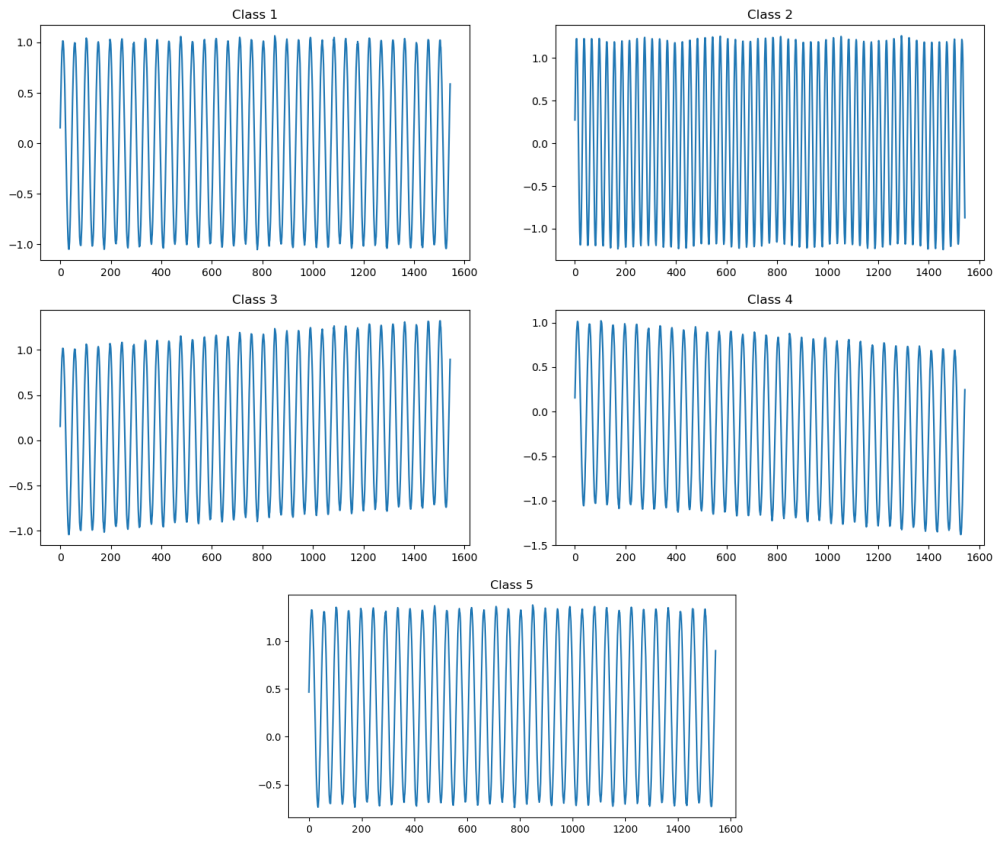
Figure 2: Example series from each class of periodic series.
