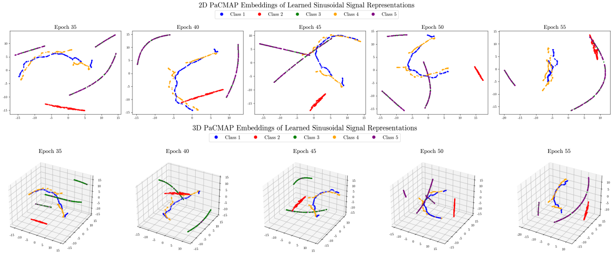
Figure 3: PaCMAP embeddings of periodic series representations in two and three dimensions.
