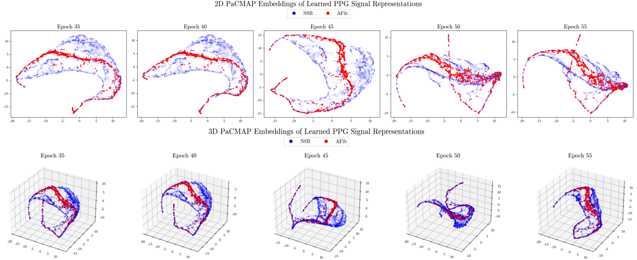
Figure 7: PaCMAP embeddings of PPG series representations in two and three dimensions.
