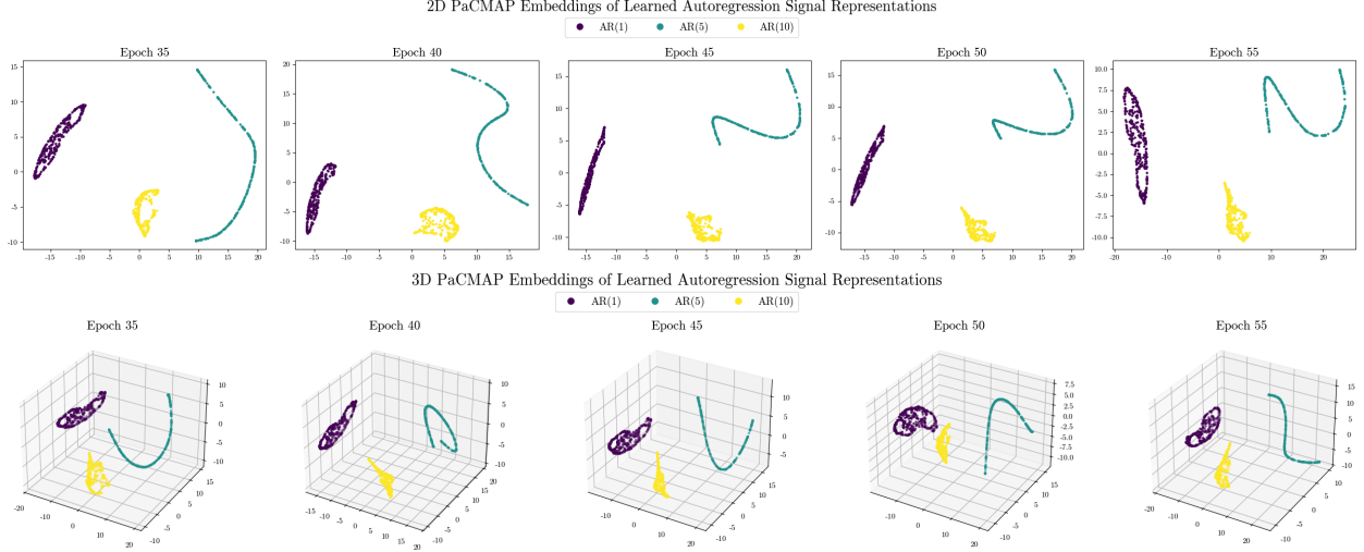
Figure 5: PaCMAP embeddings of autoregressive series representations in two and three dimensions.
