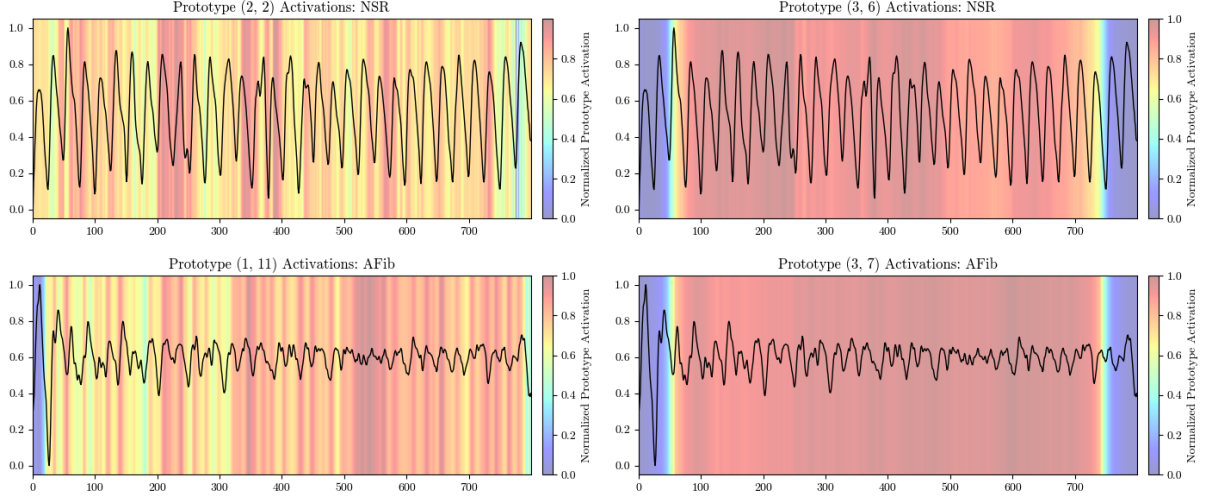
Figure 8: Highly activated prototypes for NSR (top) and AFib (bottom). Each prototype is identified by (layer, index).
