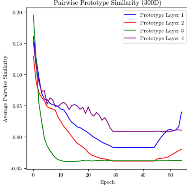
Figure 6: Average pairwise prototype similarity by layer.
