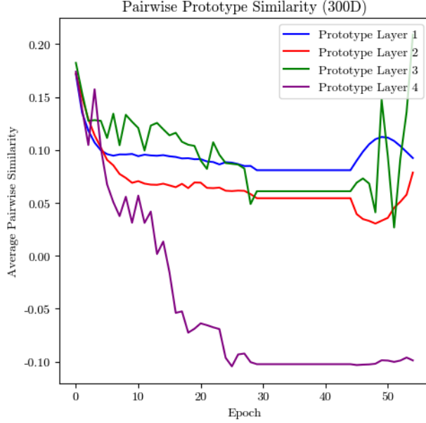
Figure 4: Average pairwise prototype similarity by layer.
