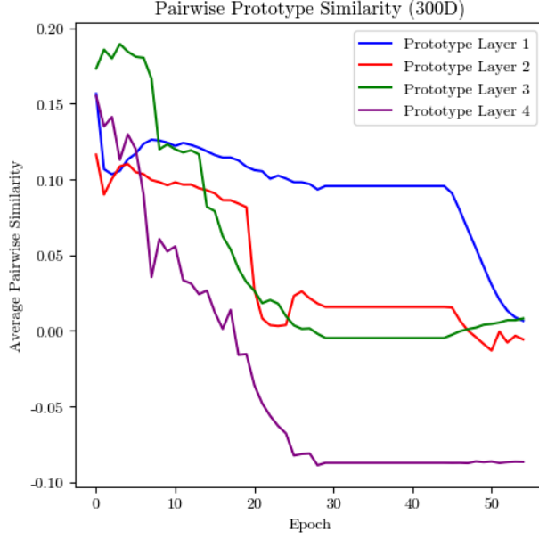
Figure 2: Average pairwise prototype similarity by layer.
