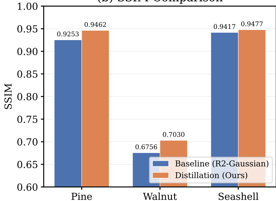
(b) SSIM Comparison
