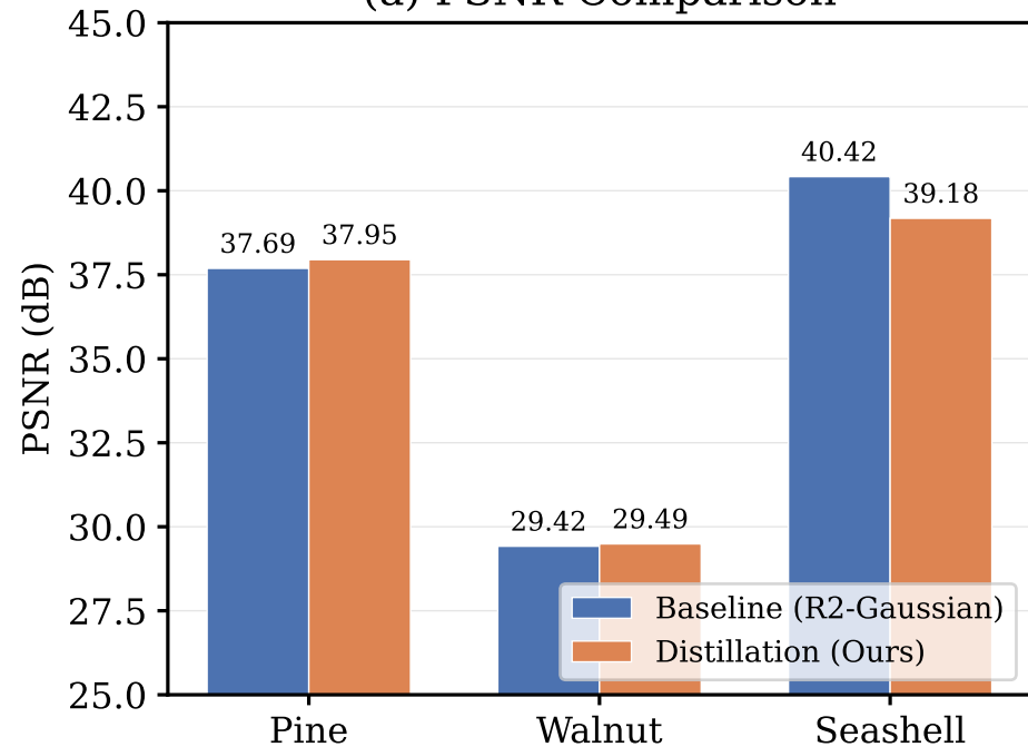
(a) PSNR Comparison
