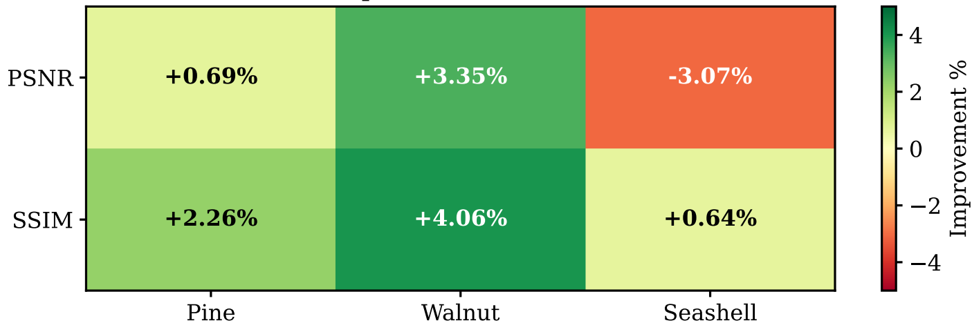
Distillation Improvement over Baseline (%)
