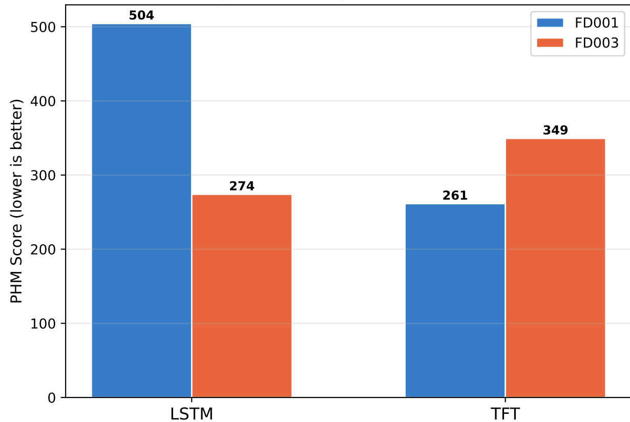
PHM Score: FD001 vs FD003 (penalizes late predictions more)
