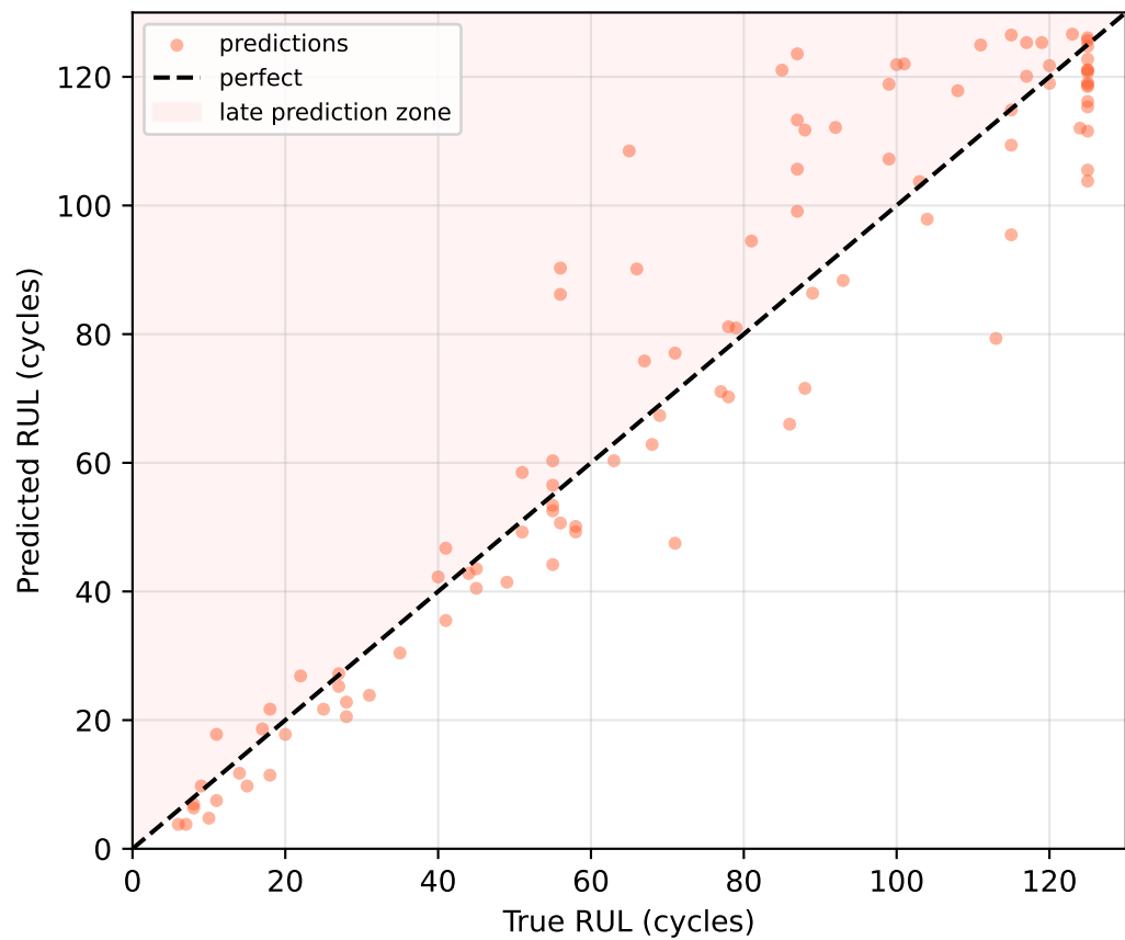
TFT / FD003 RMSE=13.04
