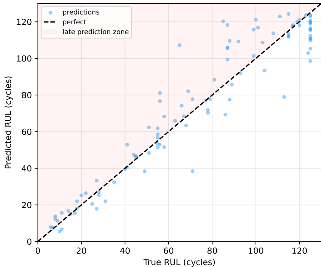
TFT / FD003 RMSE=13.04
