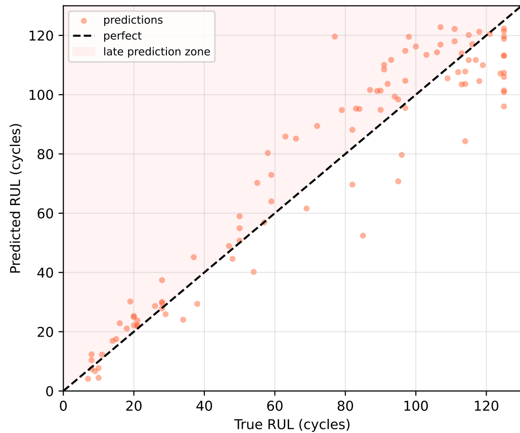
TFT / FD001 RMSE=12.63
