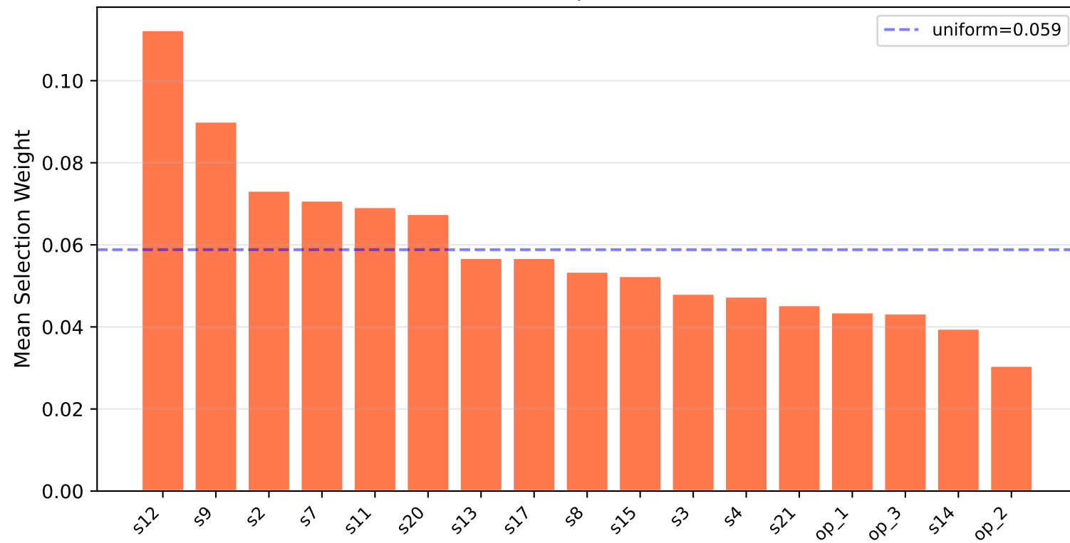
TFT Variable Importance - FD001
