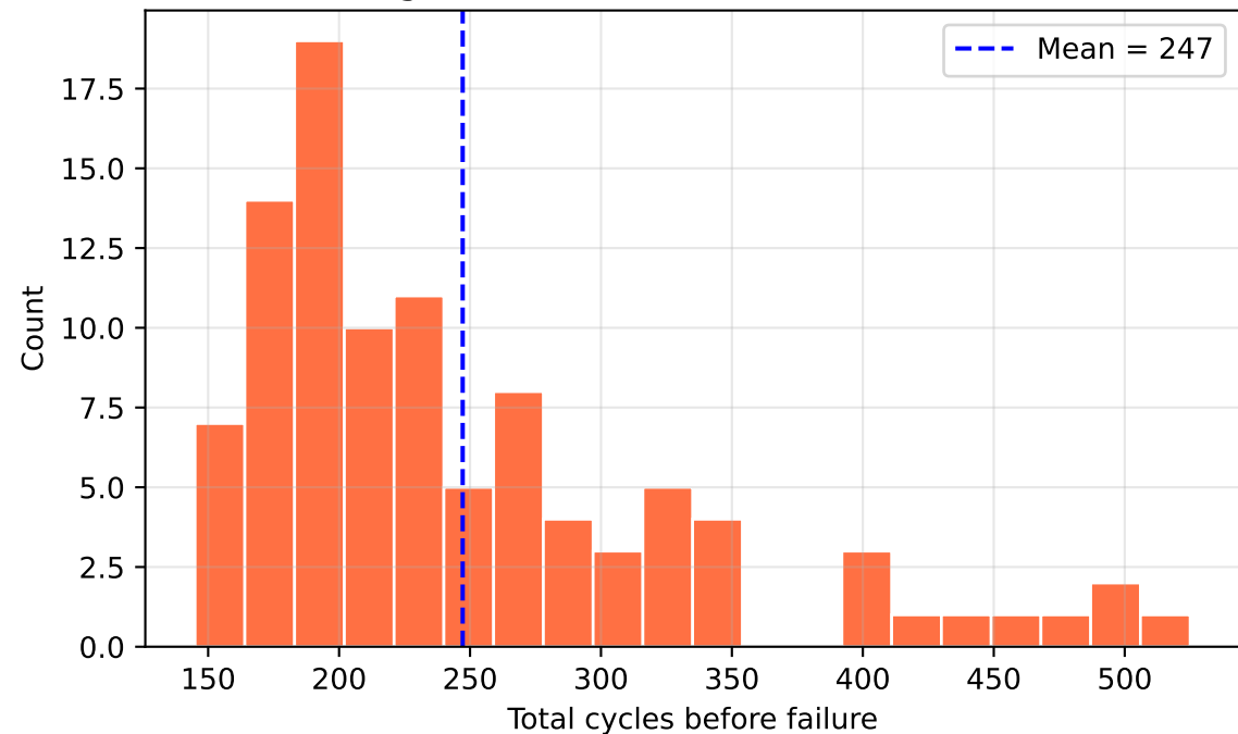
Engine Lifetime Distribution - FD003
