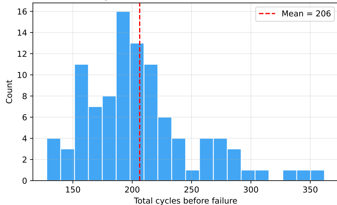
Engine Lifetime Distribution - FD001
