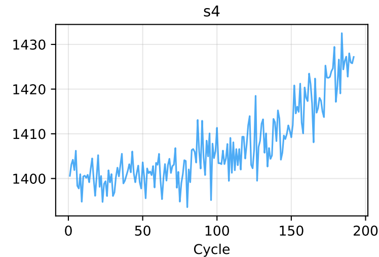
Sensor Readings Over Time for Engine 1 (FD001) - shows degradation pattern
