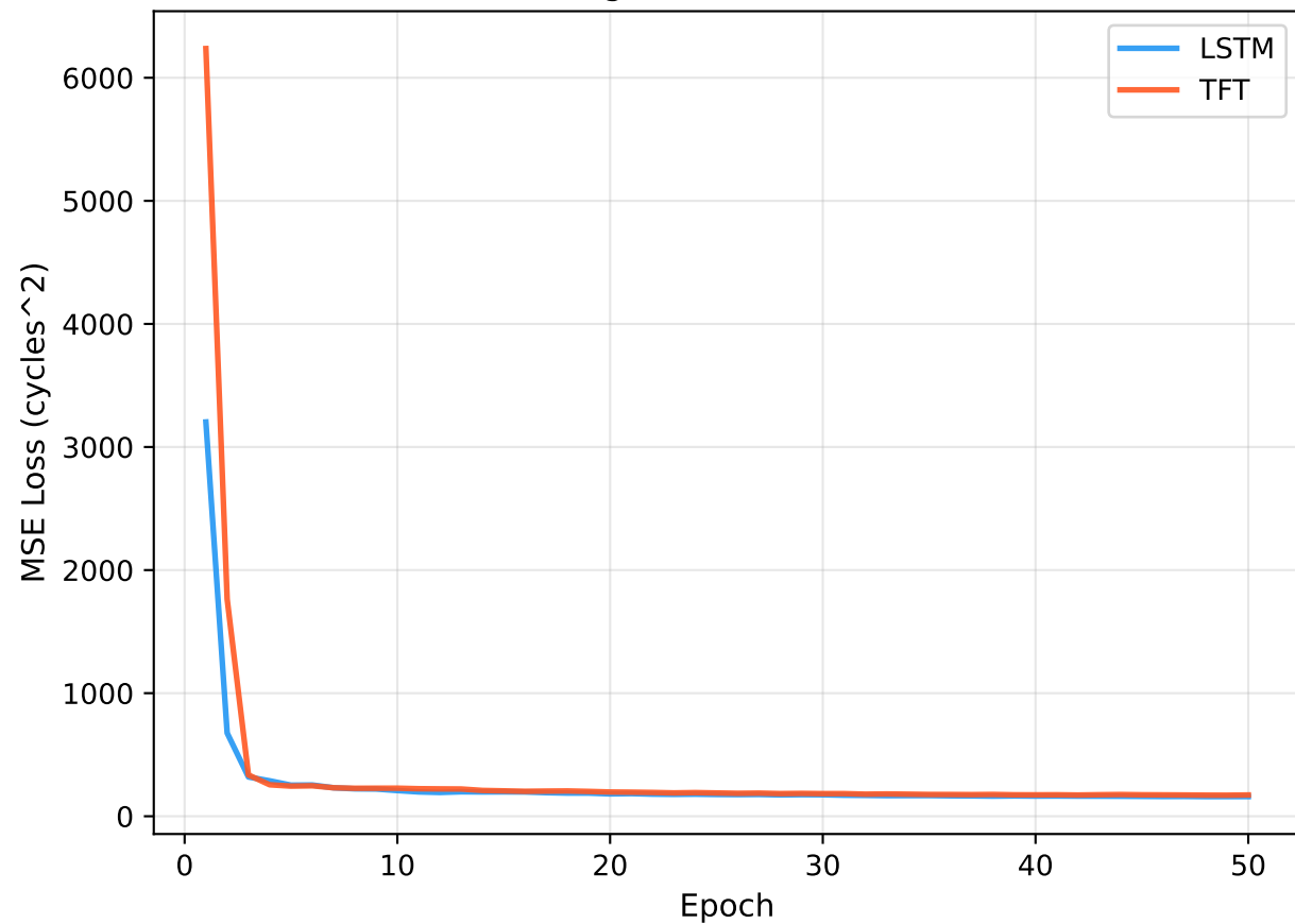
Training Loss (MSE) - FD001
