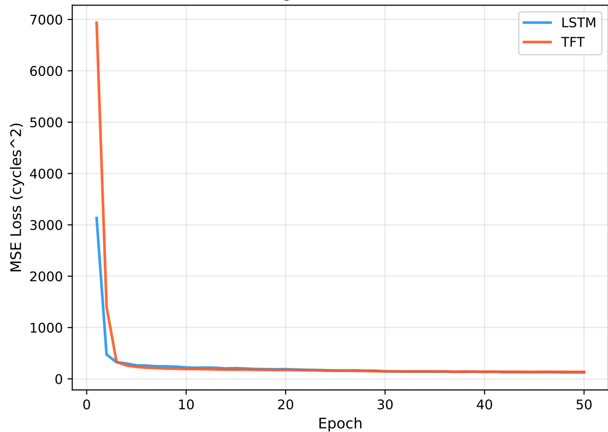
Training Loss (MSE) - FD003
